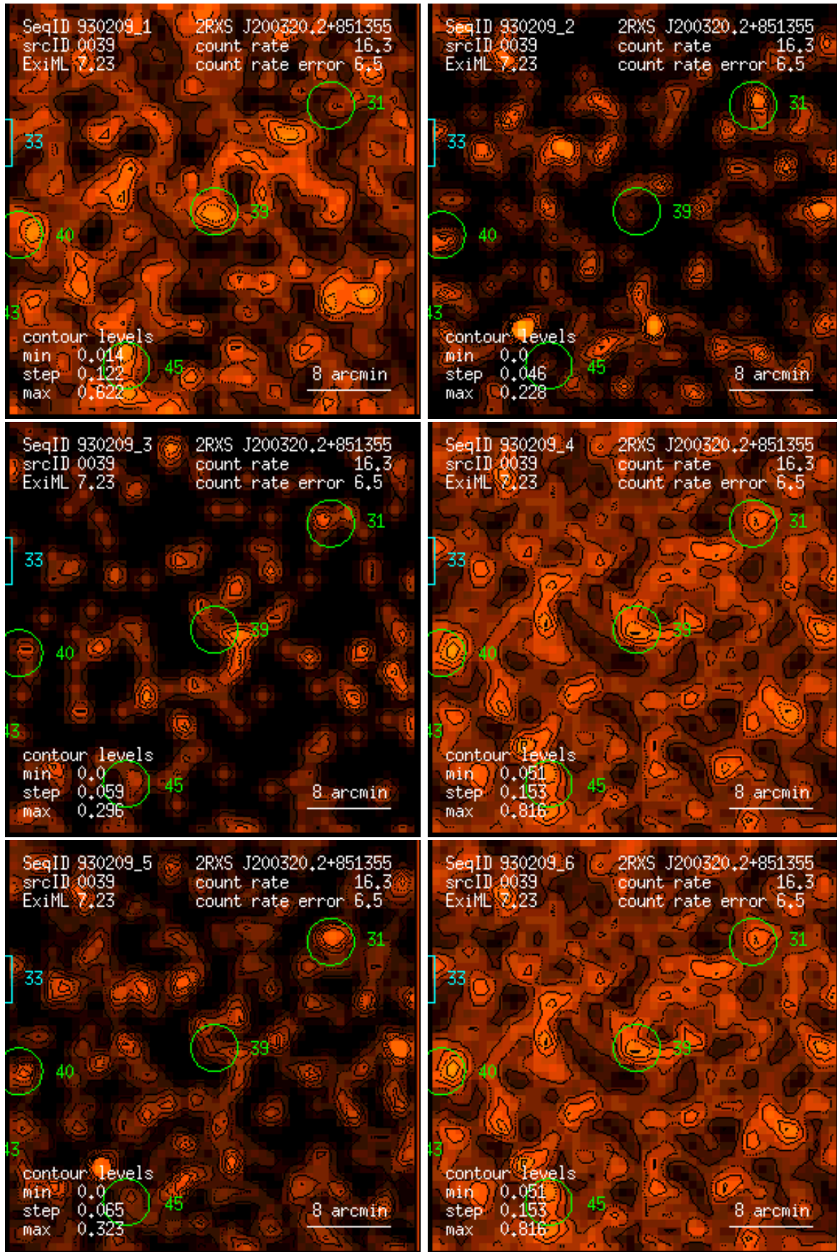
Figure 39: RASS 930209: detection 0039: band rate images, Gaussian filter: (1) PSPC channels 11 – 41, (2) 52 – 90, (3) 91 – 201, (4) 11 – 235, (5) 52 – 201, (6) 11 – 201. Broad band rates in counts/ks. Band rate contour levels in counts/ks/arcmin 2 .
