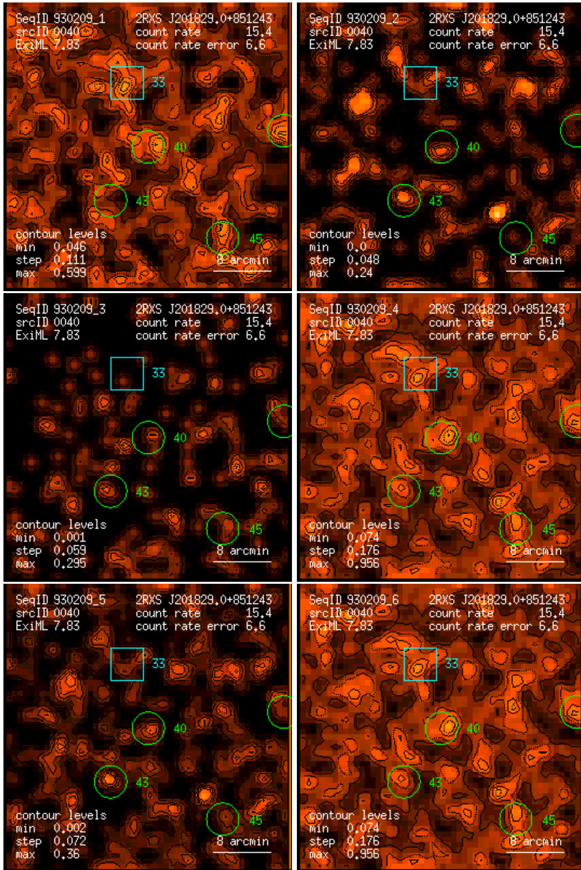
Figure 40: RASS 930209: detection 0040: band rate images, Gaussian filter: (1) PSPC channels 11 – 41, (2) 52 – 90, (3) 91 – 201, (4) 11 – 235, (5) 52 – 201, (6) 11 – 201. Broad band rates in counts/ks. Band rate contour levels in counts/ks/arcmin 2 .
