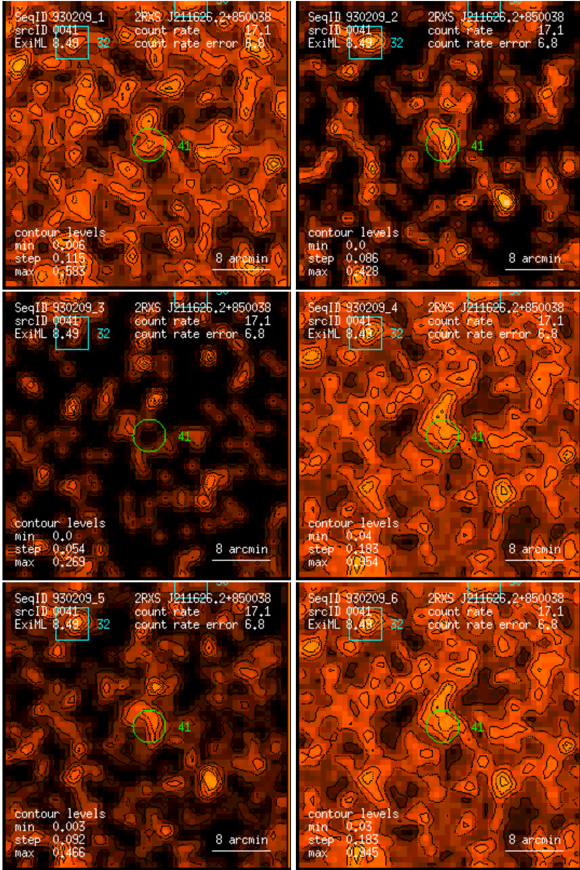
Figure 41: RASS 930209: detection 0041: band rate images, Gaussian filter: (1) PSPC channels 11 – 41, (2) 52 – 90, (3) 91 – 201, (4) 11 – 235, (5) 52 – 201, (6) 11 – 201. Broad band rates in counts/ks. Band rate contour levels in counts/ks/arcmin 2 .
