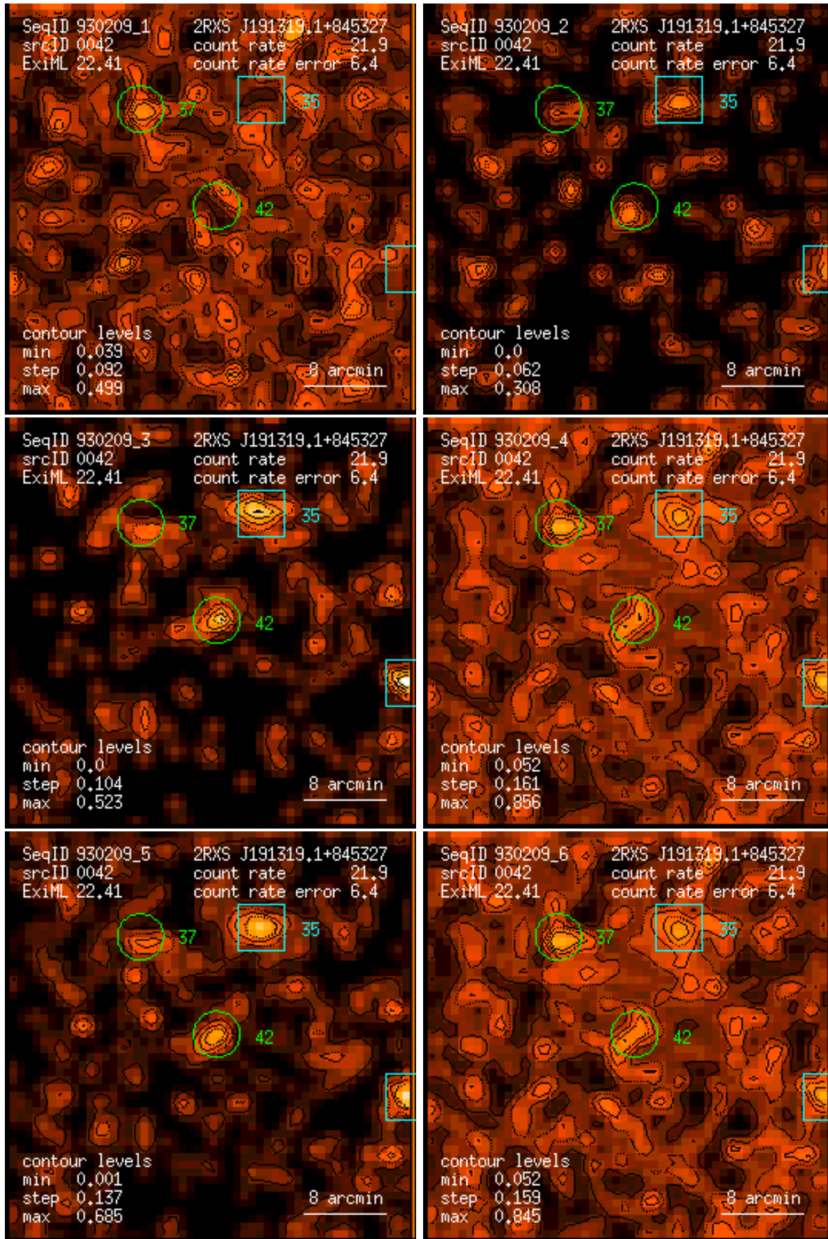
Figure 42: RASS 930209: detection 0042: band rate images, Gaussian filter: (1) PSPC channels 11 – 41, (2) 52 – 90, (3) 91 – 201, (4) 11 – 235, (5) 52 – 201, (6) 11 – 201. Broad band rates in counts/ks. Band rate contour levels in counts/ks/arcmin 2 .
