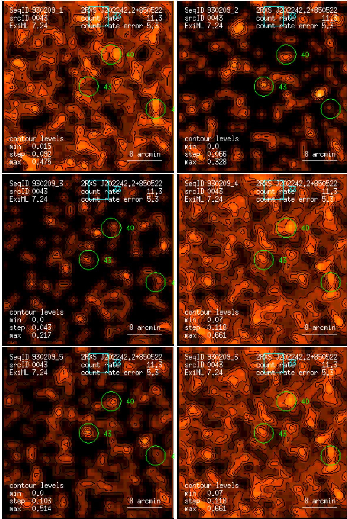
Figure 43: RASS 930209: detection 0043: band rate images, Gaussian filter: (1) PSPC channels 11 – 41, (2) 52 – 90, (3) 91 – 201, (4) 11 – 235, (5) 52 – 201, (6) 11 – 201. Broad band rates in counts/ks. Band rate contour levels in counts/ks/arcmin 2 .
