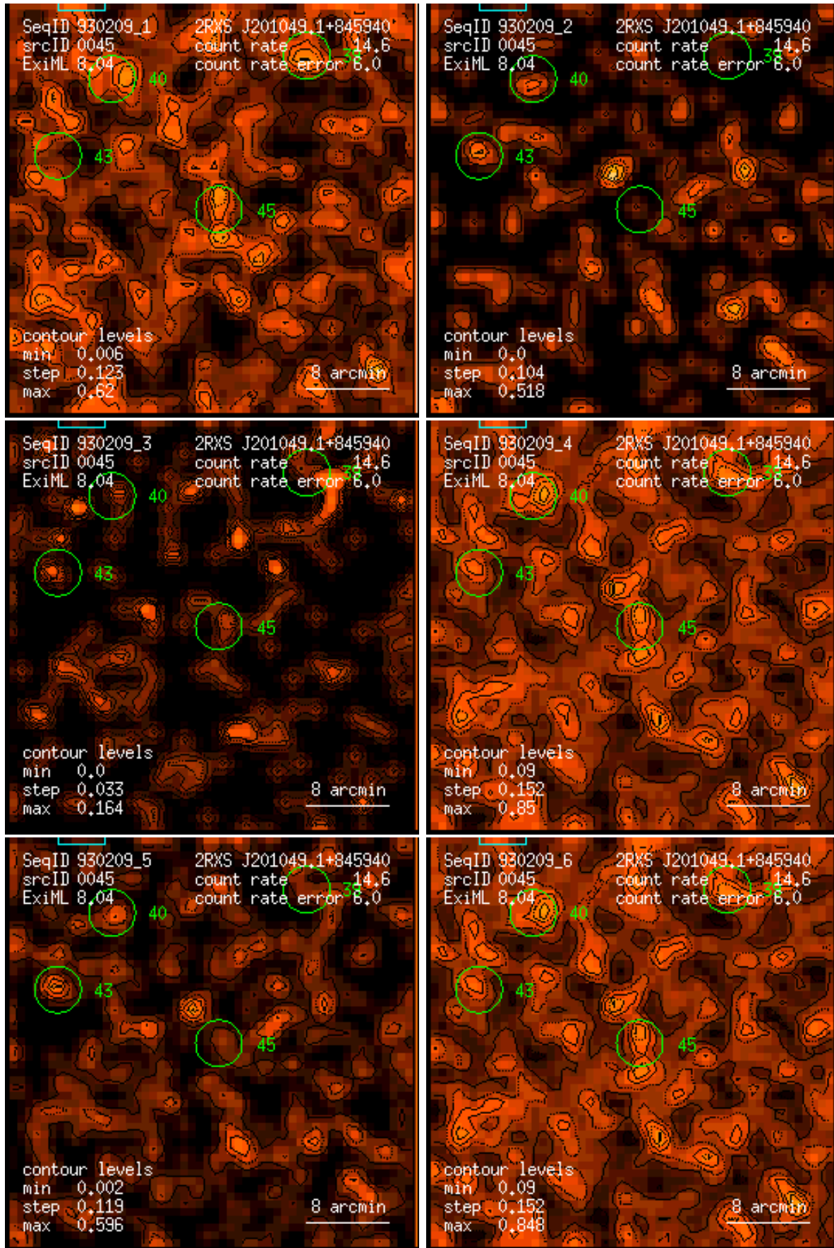
Figure 45: RASS 930209: detection 0045: band rate images, Gaussian filter: (1) PSPC channels 11 – 41, (2) 52 – 90, (3) 91 – 201, (4) 11 – 235, (5) 52 – 201, (6) 11 – 201. Broad band rates in counts/ks. Band rate contour levels in counts/ks/arcmin 2 .
