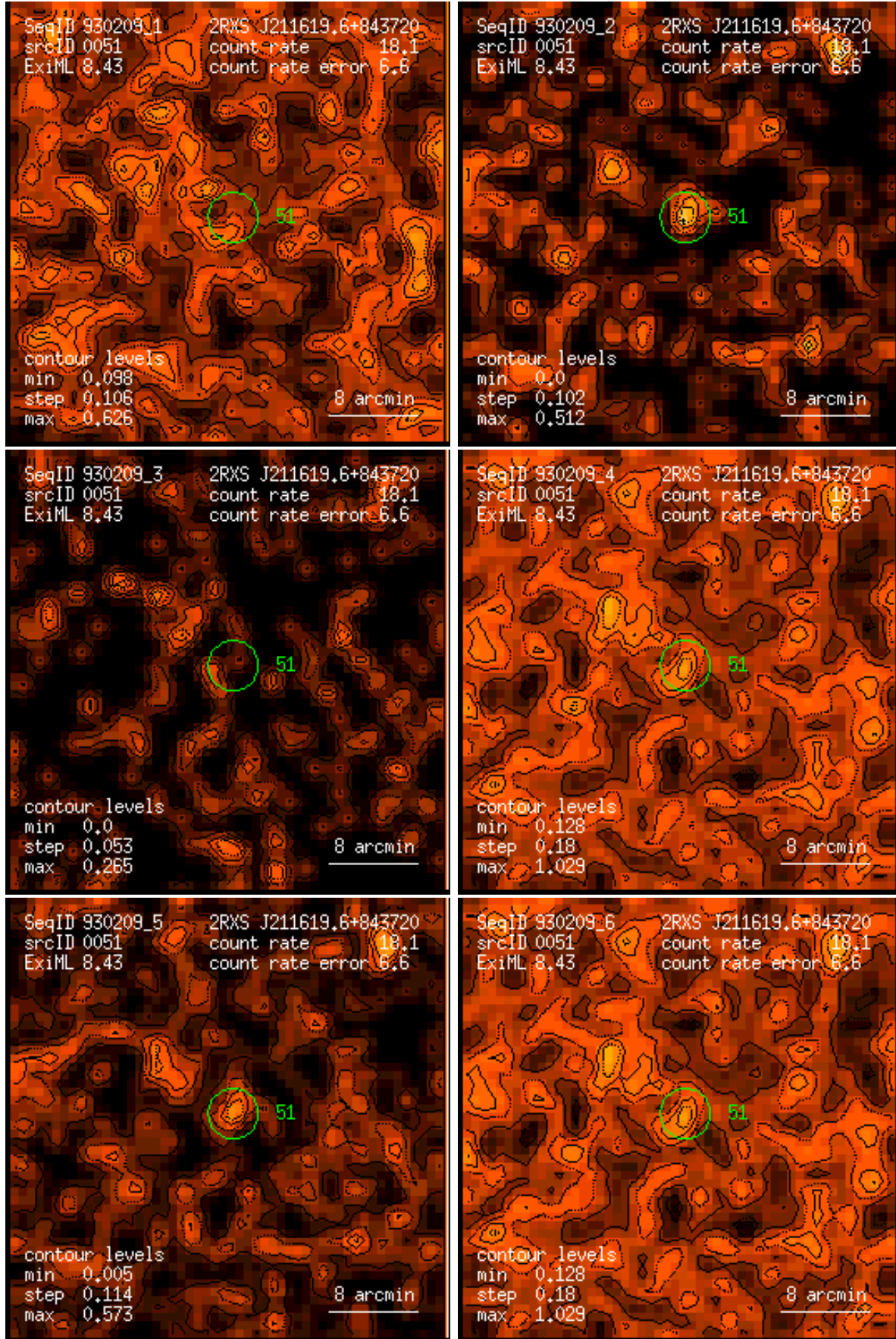
Figure 51: RASS 930209: detection 0051: band rate images, Gaussian filter: (1) PSPC channels 11 – 41, (2) 52 – 90, (3) 91 – 201, (4) 11 – 235, (5) 52 – 201, (6) 11 – 201. Broad band rates in counts/ks. Band rate contour levels in counts/ks/arcmin 2 .
