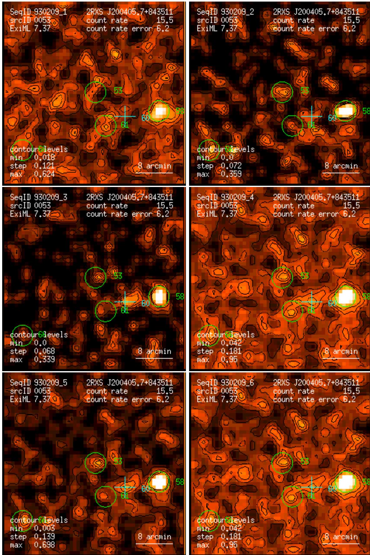
Figure 53: RASS 930209: detection 0053: band rate images, Gaussian filter: (1) PSPC channels 11 – 41, (2) 52 – 90, (3) 91 – 201, (4) 11 – 235, (5) 52 – 201, (6) 11 – 201. Broad band rates in counts/ks. Band rate contour levels in counts/ks/arcmin 2 .
