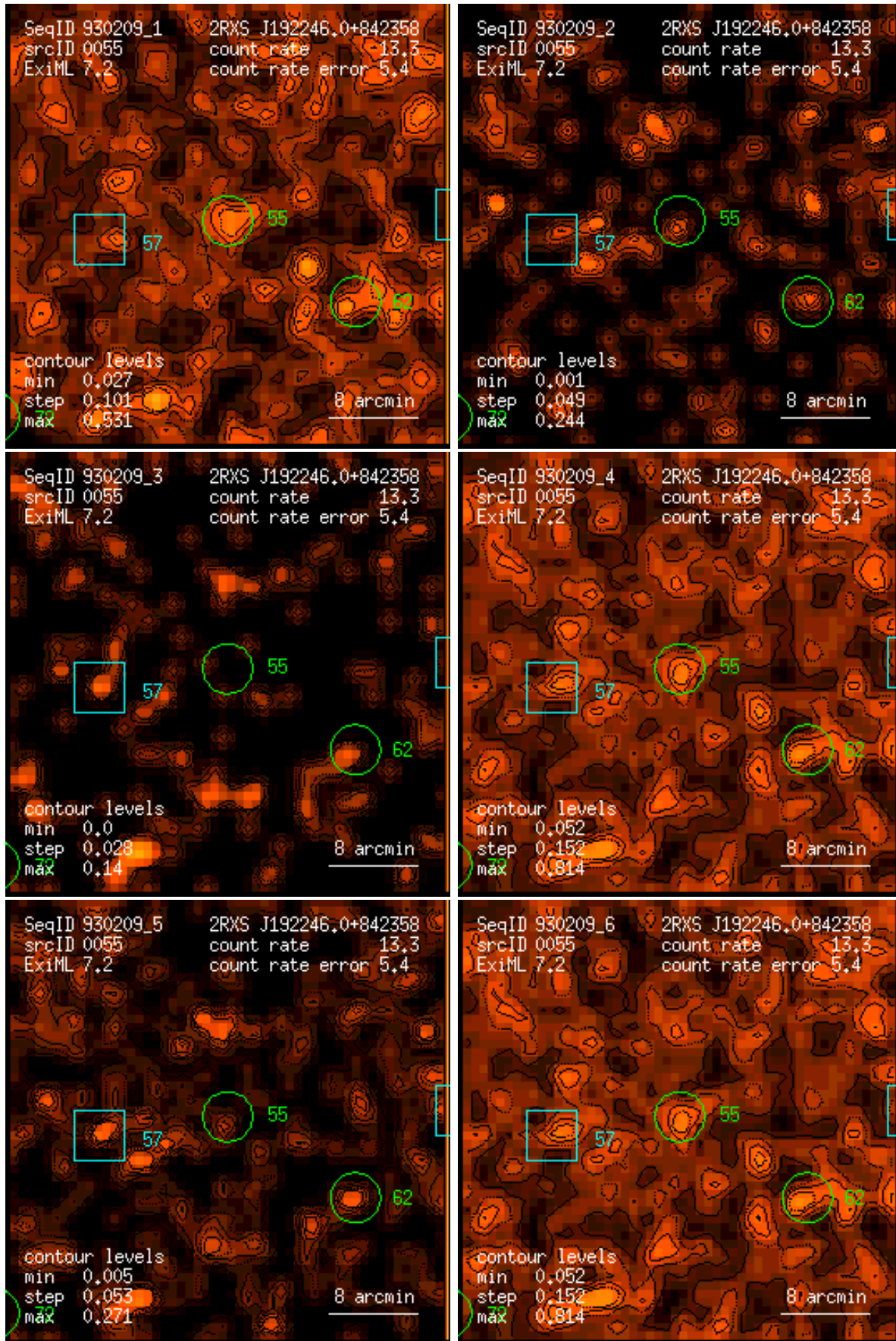
Figure 55: RASS 930209: detection 0055: band rate images, Gaussian filter: (1) PSPC channels 11 – 41, (2) 52 – 90, (3) 91 – 201, (4) 11 – 235, (5) 52 – 201, (6) 11 – 201. Broad band rates in counts/ks. Band rate contour levels in counts/ks/arcmin 2 .
