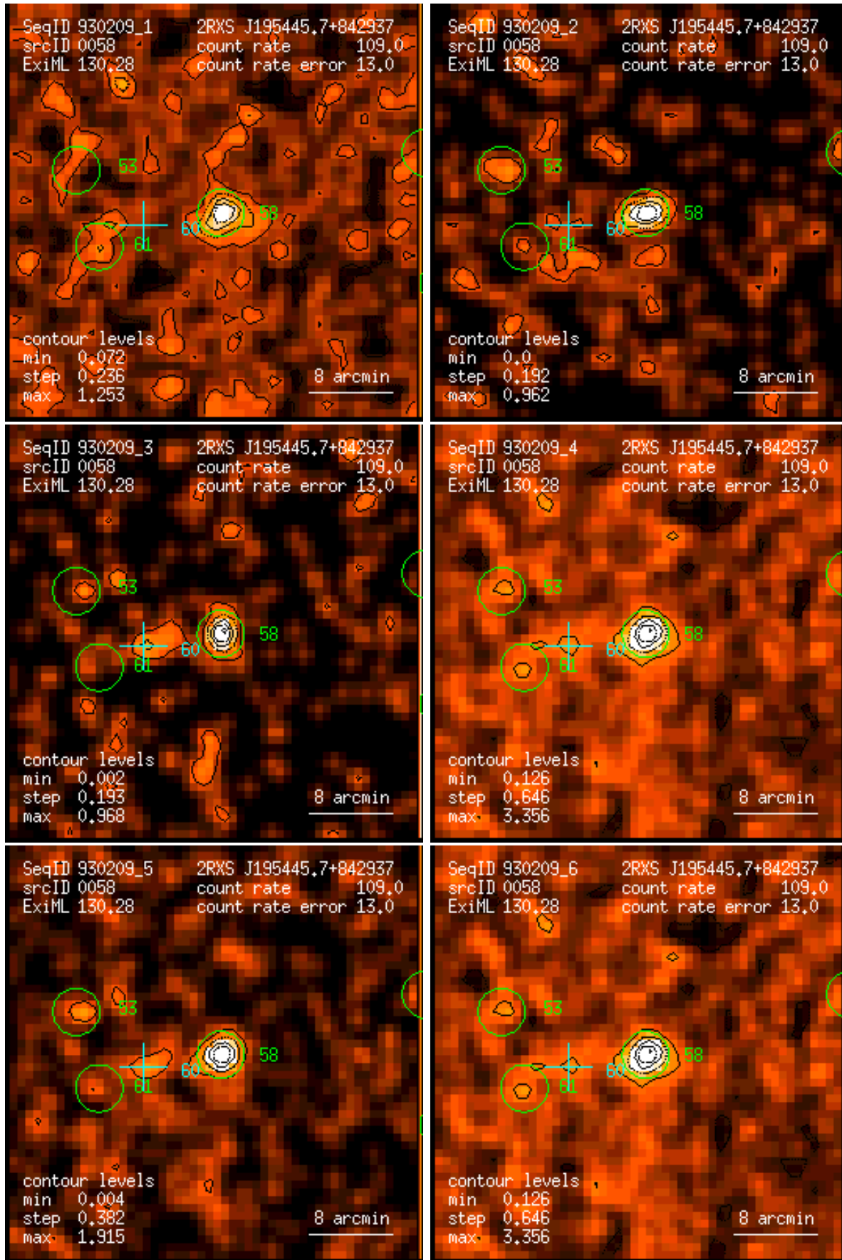
Figure 58: RASS 930209: detection 0058: band rate images, Gaussian filter: (1) PSPC channels 11 – 41, (2) 52 – 90, (3) 91 – 201, (4) 11 – 235, (5) 52 – 201, (6) 11 – 201. Broad band rates in counts/ks. Band rate contour levels in counts/ks/arcmin 2 .
