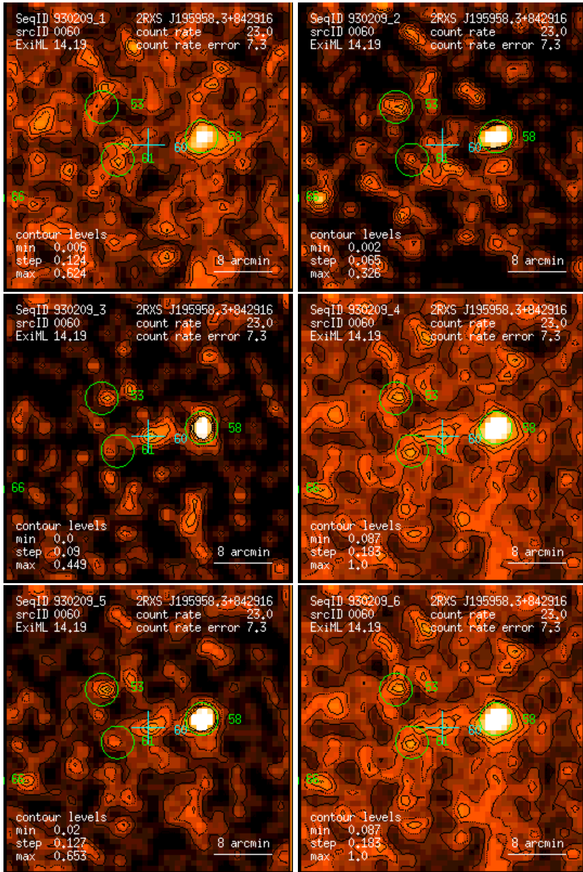
Figure 60: RASS 930209: detection 0060: band rate images, Gaussian filter: (1) PSPC channels 11 – 41, (2) 52 – 90, (3) 91 – 201, (4) 11 – 235, (5) 52 – 201, (6) 11 – 201. Broad band rates in counts/ks. Band rate contour levels in counts/ks/arcmin 2 .
