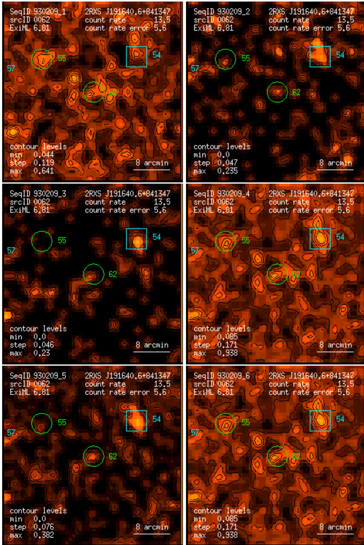
Figure 62: RASS 930209: detection 0062: band rate images, Gaussian filter: (1) PSPC channels 11 – 41, (2) 52 – 90, (3) 91 – 201, (4) 11 – 235, (5) 52 – 201, (6) 11 – 201. Broad band rates in counts/ks. Band rate contour levels in counts/ks/arcmin 2 .
