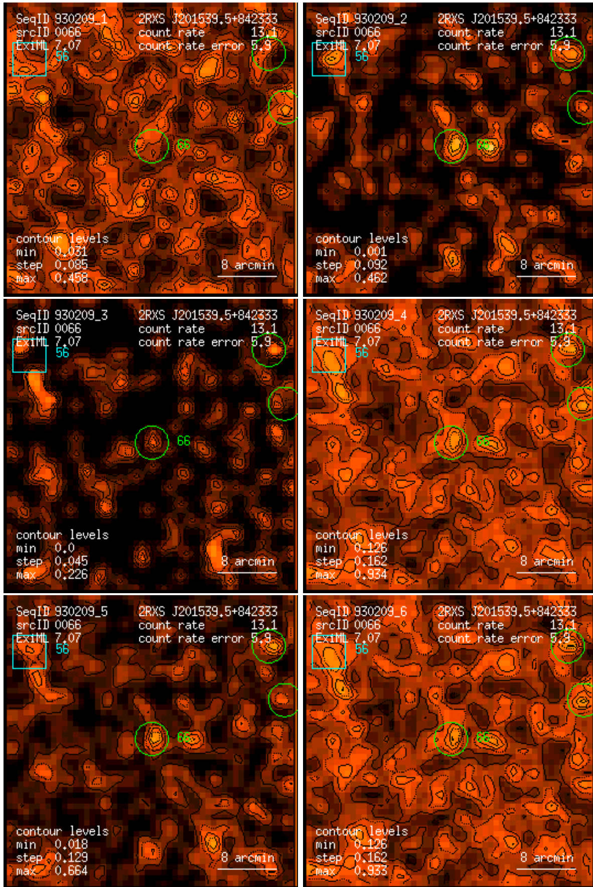
Figure 66: RASS 930209: detection 0066: band rate images, Gaussian filter: (1) PSPC channels 11 – 41, (2) 52 – 90, (3) 91 – 201, (4) 11 – 235, (5) 52 – 201, (6) 11 – 201. Broad band rates in counts/ks. Band rate contour levels in counts/ks/arcmin 2 .
