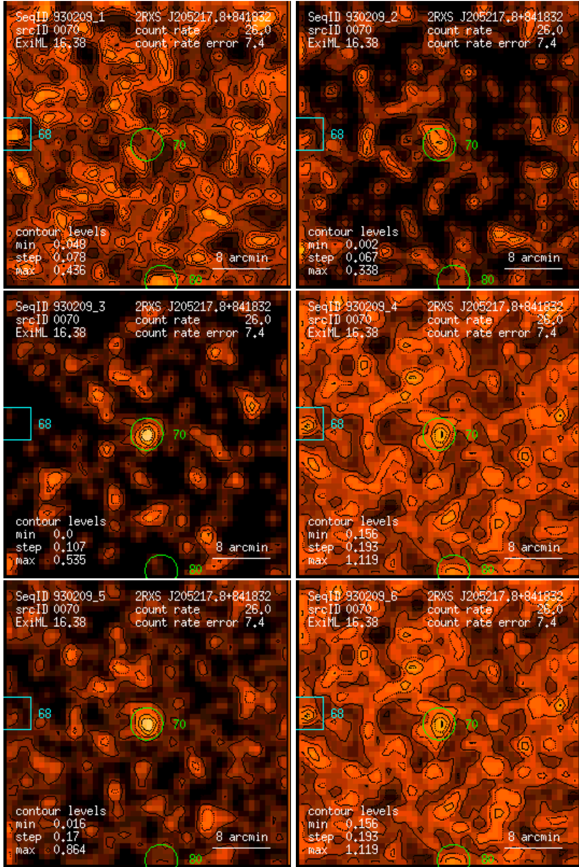
Figure 70: RASS 930209: detection 0070: band rate images, Gaussian filter: (1) PSPC channels 11 – 41, (2) 52 – 90, (3) 91 – 201, (4) 11 – 235, (5) 52 – 201, (6) 11 – 201. Broad band rates in counts/ks. Band rate contour levels in counts/ks/arcmin 2 .
