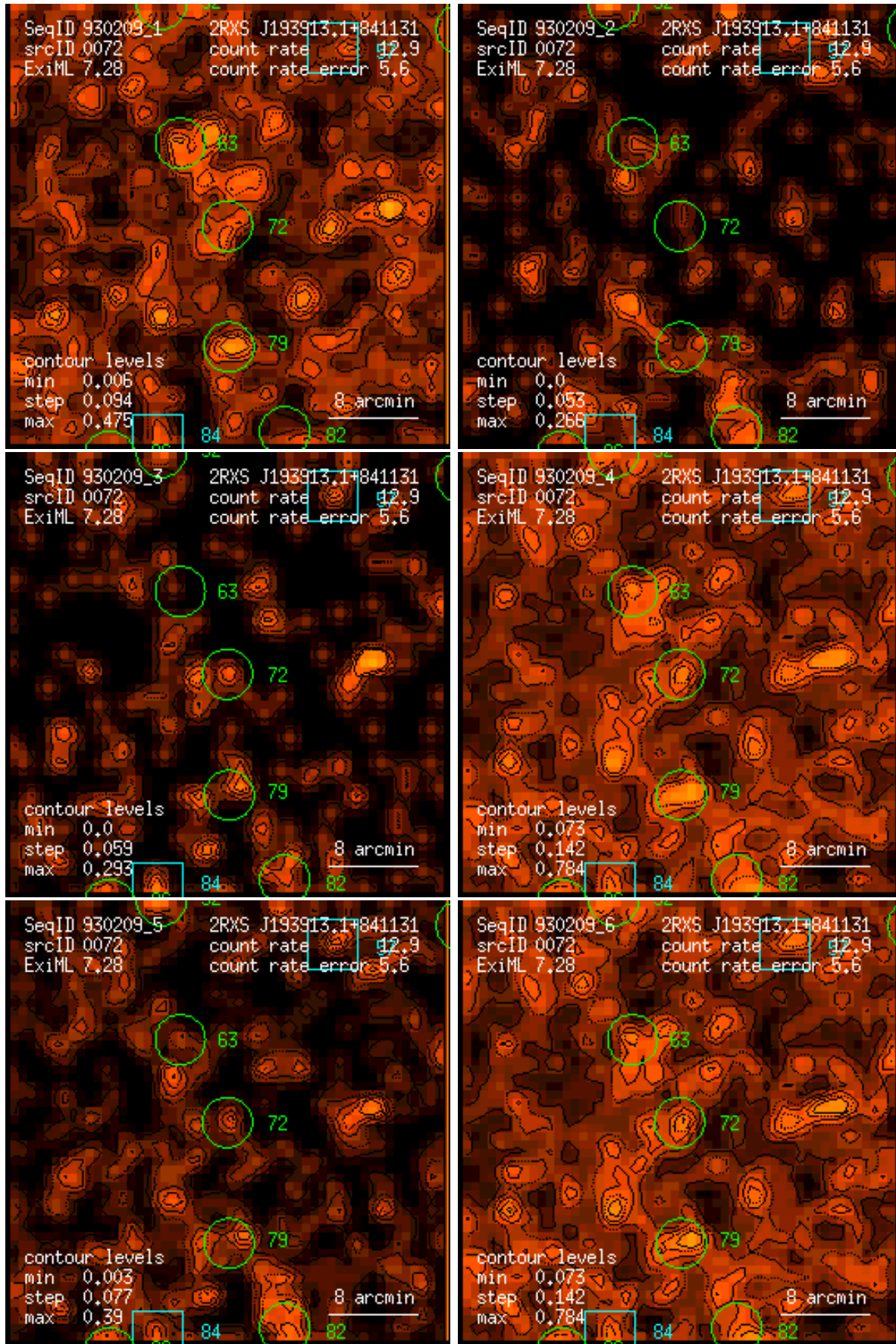
Figure 72: RASS 930209: detection 0072: band rate images, Gaussian filter: (1) PSPC channels 11 – 41, (2) 52 – 90, (3) 91 – 201, (4) 11 – 235, (5) 52 – 201, (6) 11 – 201. Broad band rates in counts/ks. Band rate contour levels in counts/ks/arcmin 2 .
