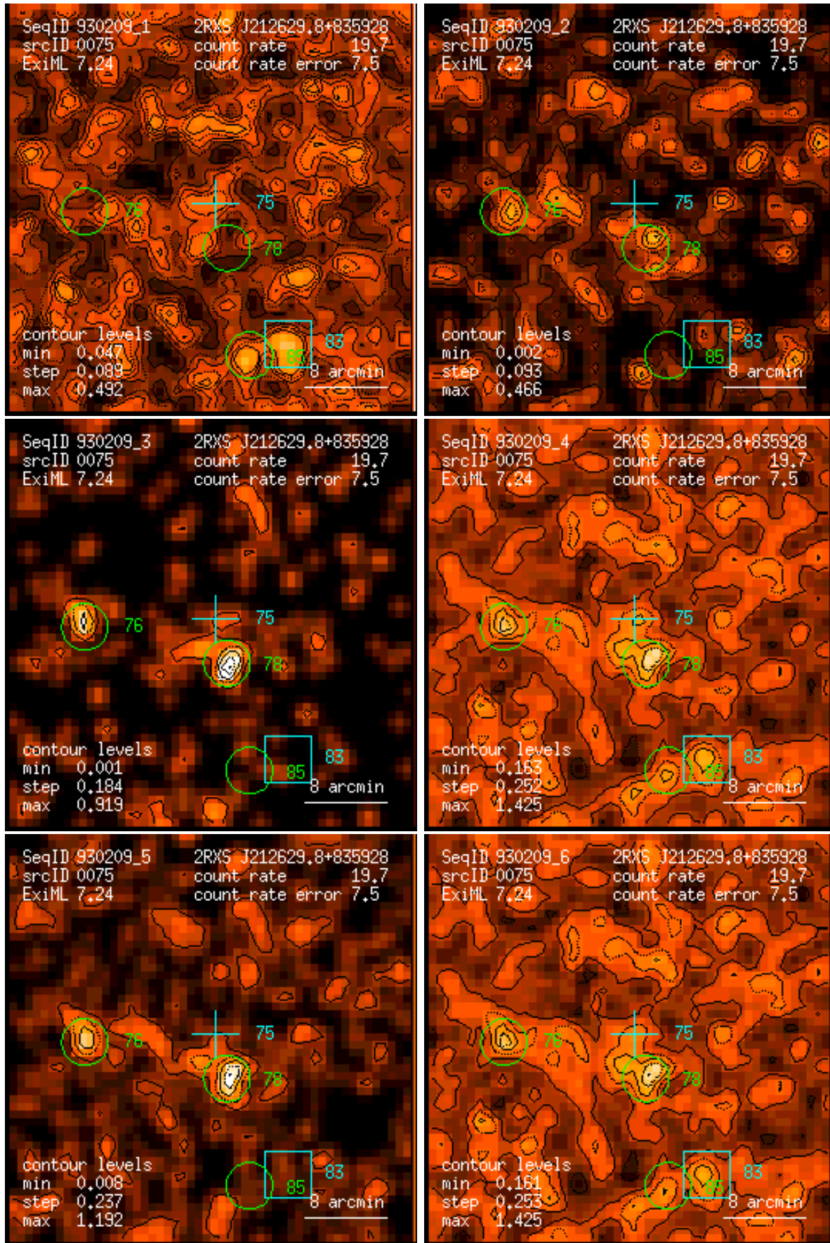
Figure 75: RASS 930209: detection 0075: band rate images, Gaussian filter: (1) PSPC channels 11 – 41, (2) 52 – 90, (3) 91 – 201, (4) 11 – 235, (5) 52 – 201, (6) 11 – 201. Broad band rates in counts/ks. Band rate contour levels in counts/ks/arcmin 2 .
