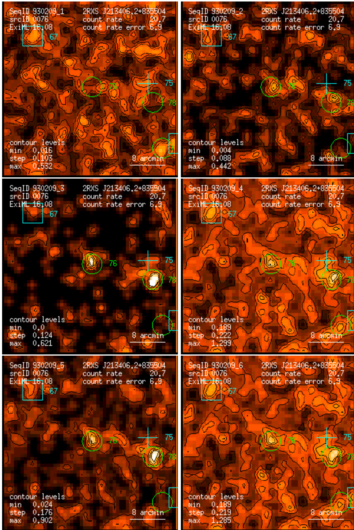
Figure 76: RASS 930209: detection 0076: band rate images, Gaussian filter: (1) PSPC channels 11 – 41, (2) 52 – 90, (3) 91 – 201, (4) 11 – 235, (5) 52 – 201, (6) 11 – 201. Broad band rates in counts/ks. Band rate contour levels in counts/ks/arcmin 2 .
