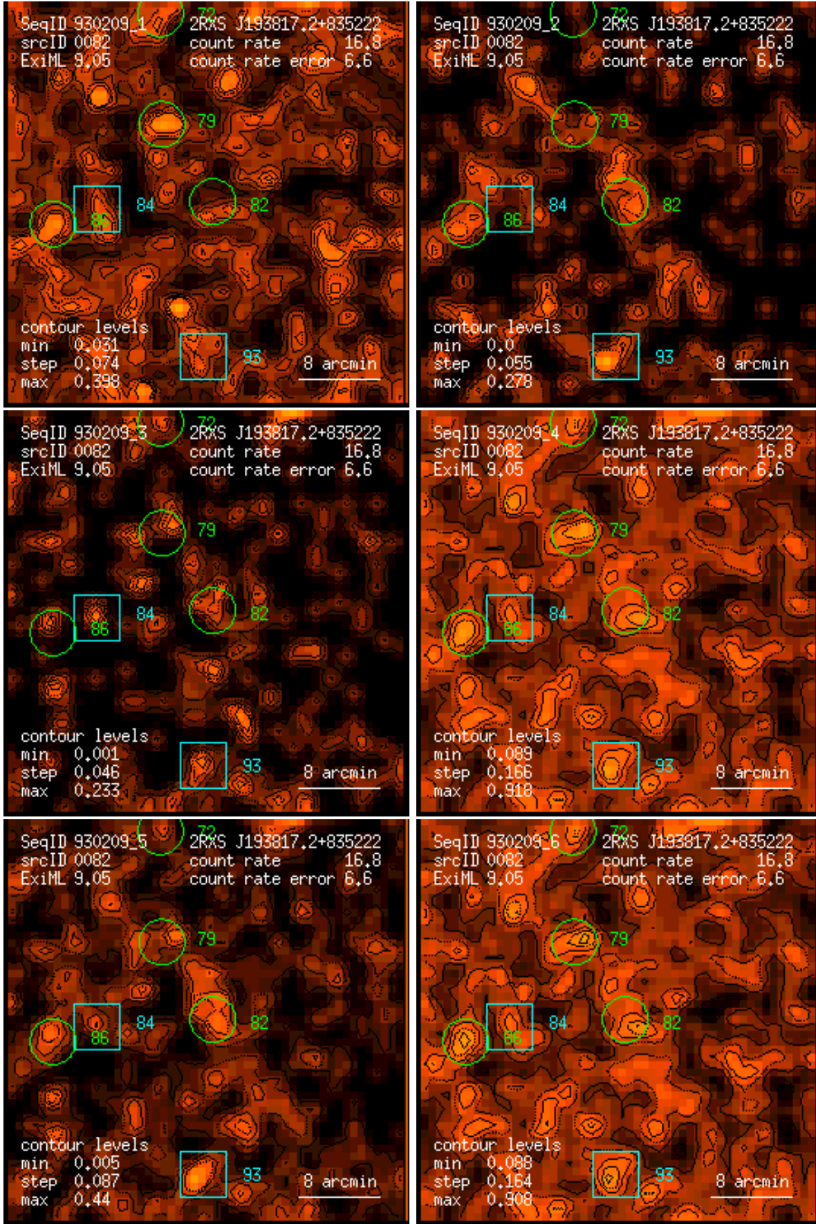
Figure 82: RASS 930209: detection 0082: band rate images, Gaussian filter: (1) PSPC channels 11 – 41, (2) 52 – 90, (3) 91 – 201, (4) 11 – 235, (5) 52 – 201, (6) 11 – 201. Broad band rates in counts/ks. Band rate contour levels in counts/ks/arcmin 2 .
