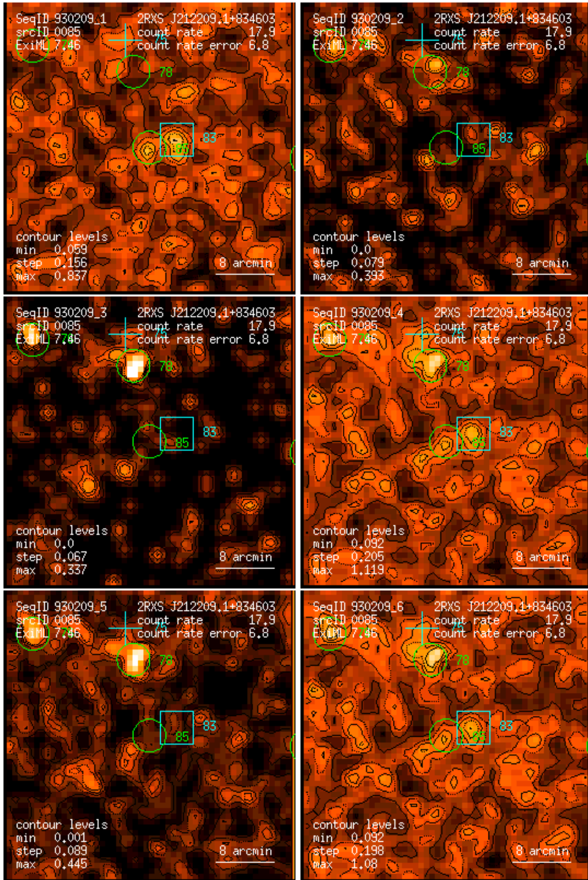
Figure 85: RASS 930209: detection 0085: band rate images, Gaussian filter: (1) PSPC channels 11 – 41, (2) 52 – 90, (3) 91 – 201, (4) 11 – 235, (5) 52 – 201, (6) 11 – 201. Broad band rates in counts/ks. Band rate contour levels in counts/ks/arcmin 2 .
