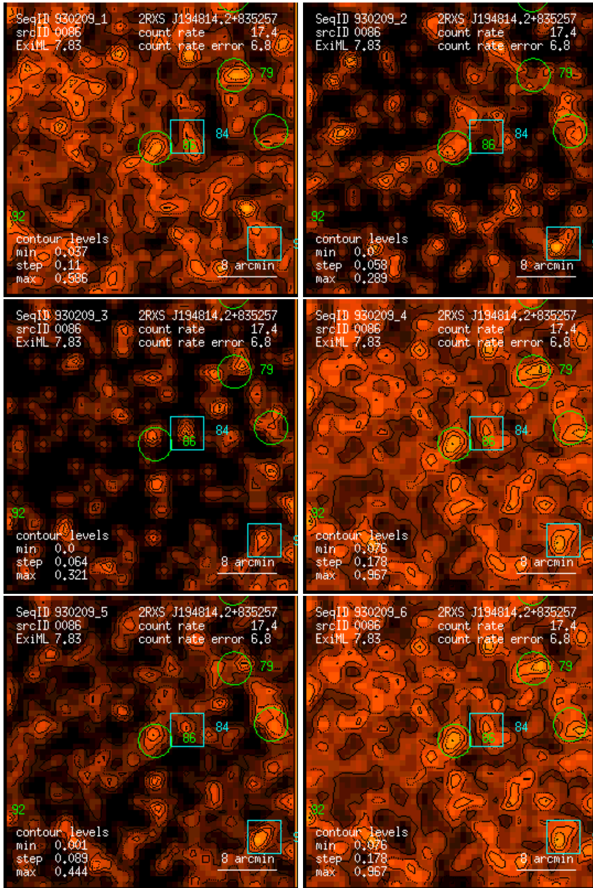
Figure 86: RASS 930209: detection 0086: band rate images, Gaussian filter: (1) PSPC channels 11 – 41, (2) 52 – 90, (3) 91 – 201, (4) 11 – 235, (5) 52 – 201, (6) 11 – 201. Broad band rates in counts/ks. Band rate contour levels in counts/ks/arcmin 2 .
