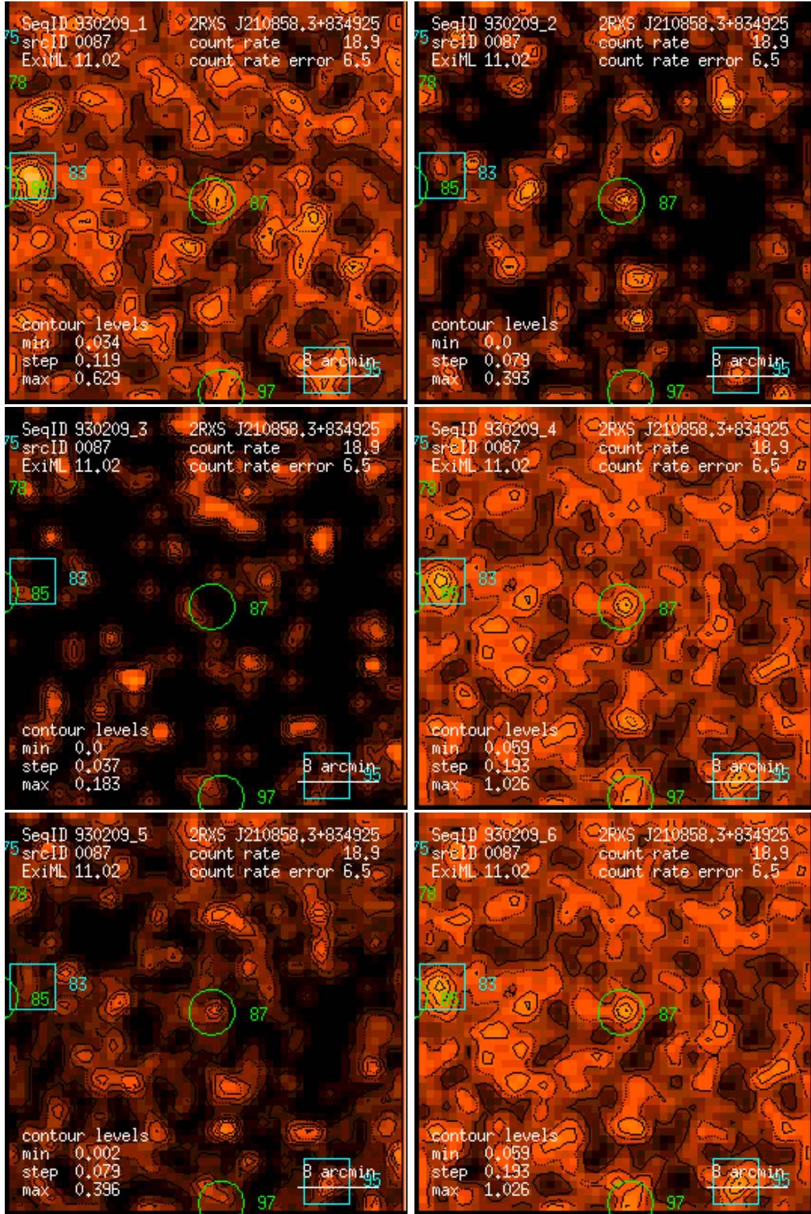
Figure 87: RASS 930209: detection 0087: band rate images, Gaussian filter: (1) PSPC channels 11 – 41, (2) 52 – 90, (3) 91 – 201, (4) 11 – 235, (5) 52 – 201, (6) 11 – 201. Broad band rates in counts/ks. Band rate contour levels in counts/ks/arcmin 2 .
