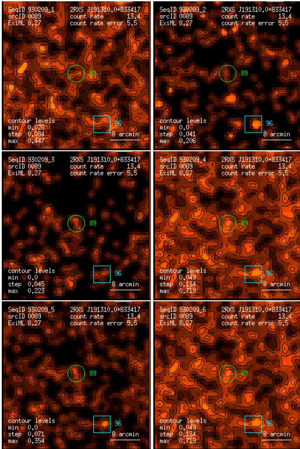
Figure 89: RASS 930209: detection 0089: band rate images, Gaussian filter: (1) PSPC channels 11 – 41, (2) 52 – 90, (3) 91 – 201, (4) 11 – 235, (5) 52 – 201, (6) 11 – 201. Broad band rates in counts/ks. Band rate contour levels in counts/ks/arcmin 2 .
