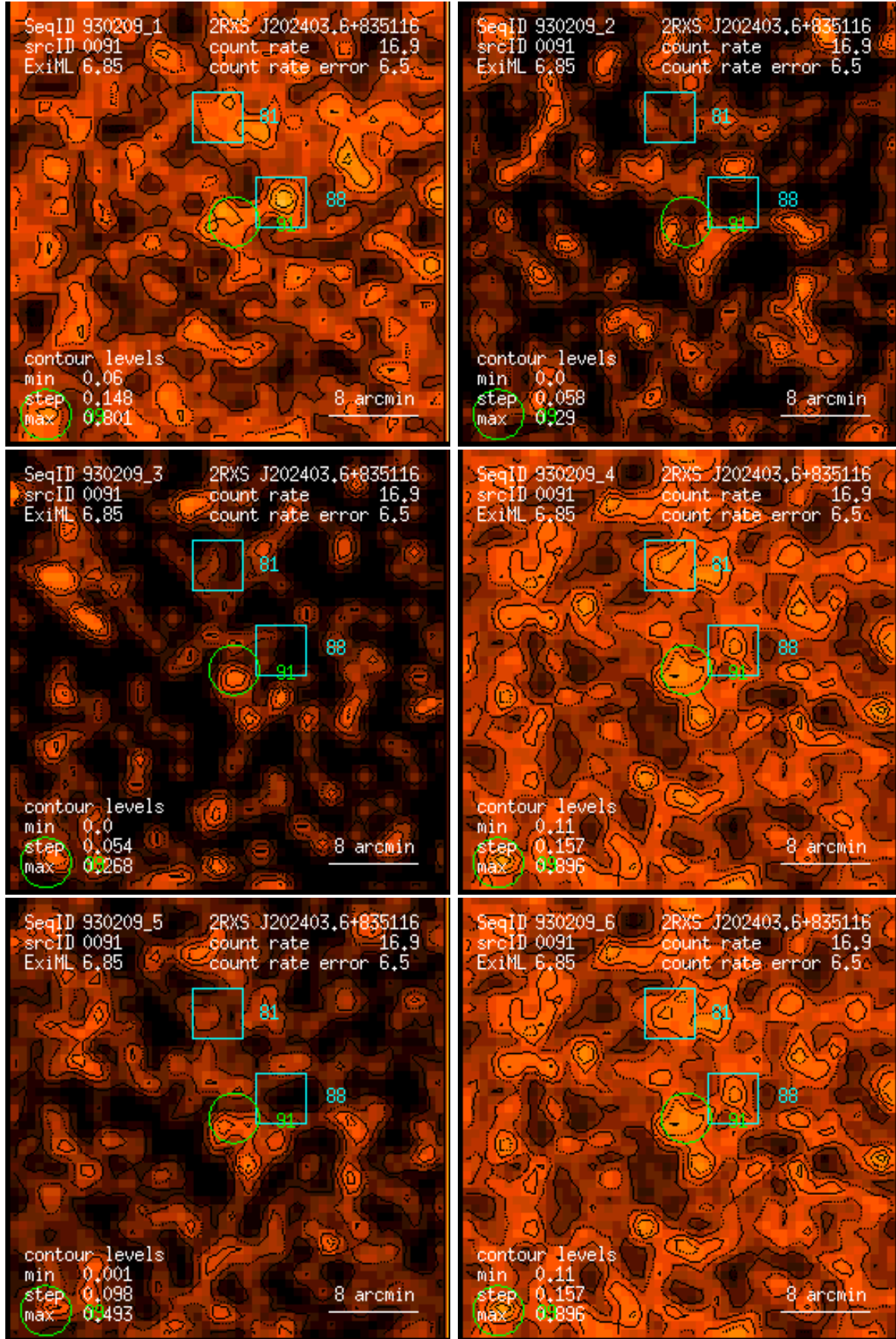
Figure 91: RASS 930209: detection 0091: band rate images, Gaussian filter: (1) PSPC channels 11 – 41, (2) 52 – 90, (3) 91 – 201, (4) 11 – 235, (5) 52 – 201, (6) 11 – 201. Broad band rates in counts/ks. Band rate contour levels in counts/ks/arcmin 2 .
