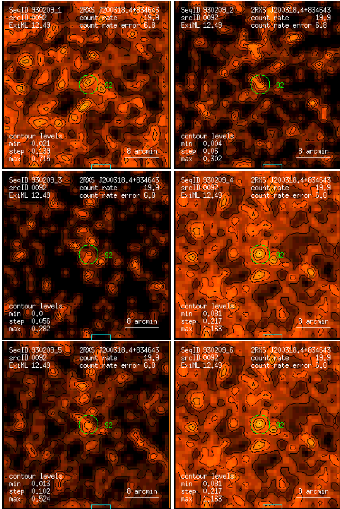
Figure 92: RASS 930209: detection 0092: band rate images, Gaussian filter: (1) PSPC channels 11 – 41, (2) 52 – 90, (3) 91 – 201, (4) 11 – 235, (5) 52 – 201, (6) 11 – 201. Broad band rates in counts/ks. Band rate contour levels in counts/ks/arcmin 2 .
