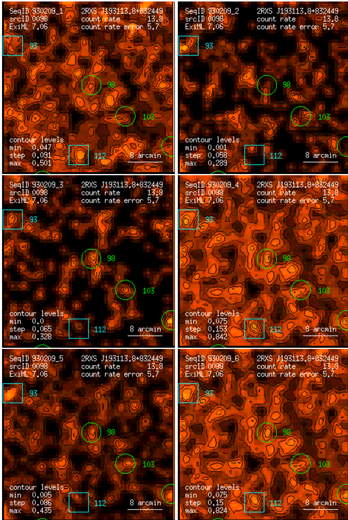
Figure 98: RASS 930209: detection 0098: band rate images, Gaussian filter: (1) PSPC channels 11 – 41, (2) 52 – 90, (3) 91 – 201, (4) 11 – 235, (5) 52 – 201, (6) 11 – 201. Broad band rates in counts/ks. Band rate contour levels in counts/ks/arcmin 2 .
