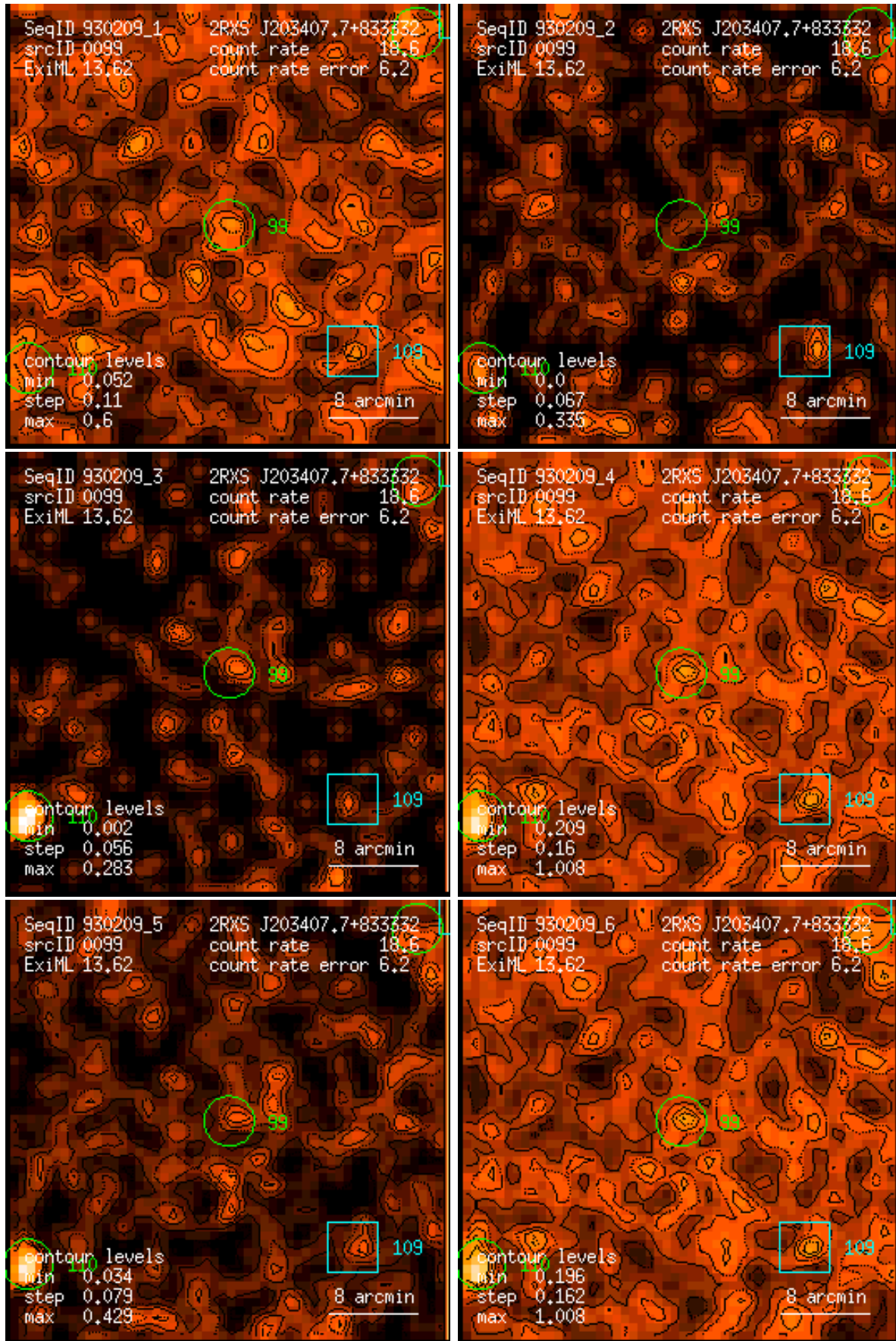
Figure 99: RASS 930209: detection 0099: band rate images, Gaussian filter: (1) PSPC channels 11 – 41, (2) 52 – 90, (3) 91 – 201, (4) 11 – 235, (5) 52 – 201, (6) 11 – 201. Broad band rates in counts/ks. Band rate contour levels in counts/ks/arcmin 2 .
