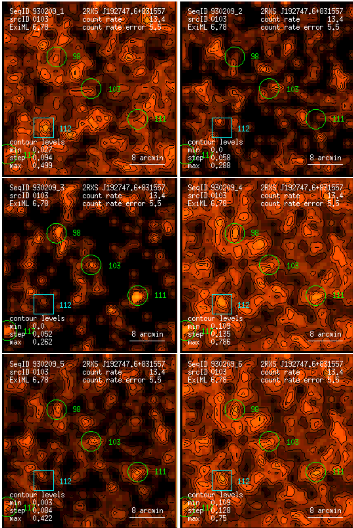
Figure 103: RASS 930209: detection 0103: band rate images, Gaussian filter: (1) PSPC channels 11 – 41, (2) 52 – 90, (3) 91 – 201, (4) 11 – 235, (5) 52 – 201, (6) 11 – 201. Broad band rates in counts/ks. Band rate contour levels in counts/ks/arcmin 2 .
