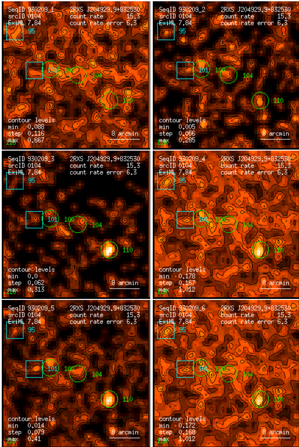
Figure 104: RASS 930209: detection 0104: band rate images, Gaussian filter: (1) PSPC channels 11 – 41, (2) 52 – 90, (3) 91 – 201, (4) 11 – 235, (5) 52 – 201, (6) 11 – 201. Broad band rates in counts/ks. Band rate contour levels in counts/ks/arcmin 2 .
