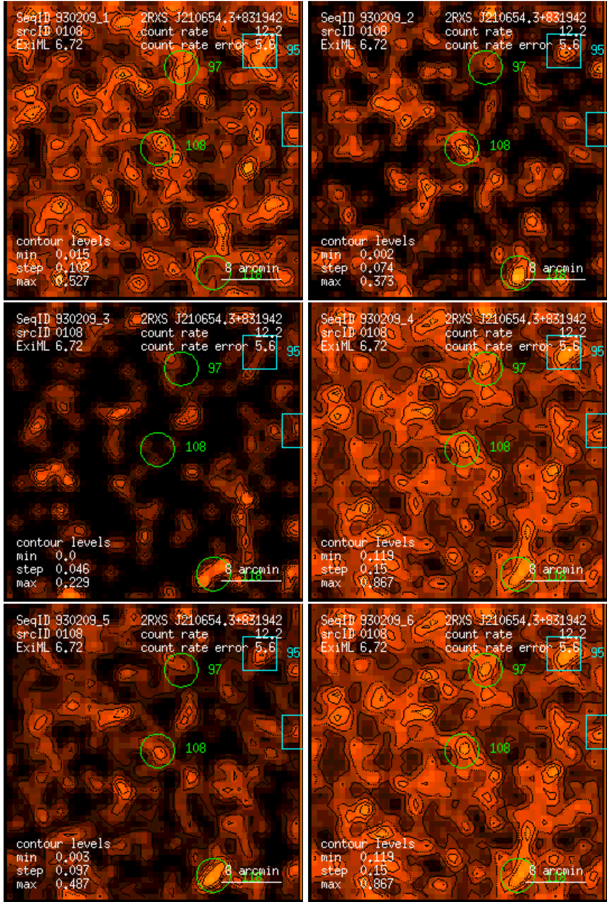
Figure 108: RASS 930209: detection 0108: band rate images, Gaussian filter: (1) PSPC channels 11 – 41, (2) 52 – 90, (3) 91 – 201, (4) 11 – 235, (5) 52 – 201, (6) 11 – 201. Broad band rates in counts/ks. Band rate contour levels in counts/ks/arcmin 2 .
