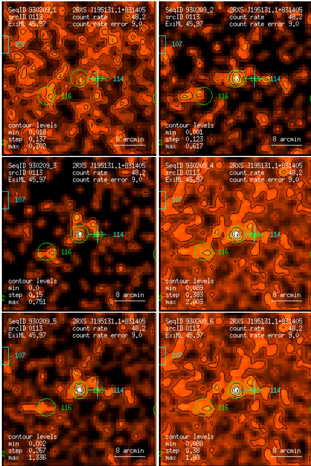
Figure 113: RASS 930209: detection 0113: band rate images, Gaussian filter: (1) PSPC channels 11 – 41, (2) 52 – 90, (3) 91 – 201, (4) 11 – 235, (5) 52 – 201, (6) 11 – 201. Broad band rates in counts/ks. Band rate contour levels in counts/ks/arcmin 2 .
