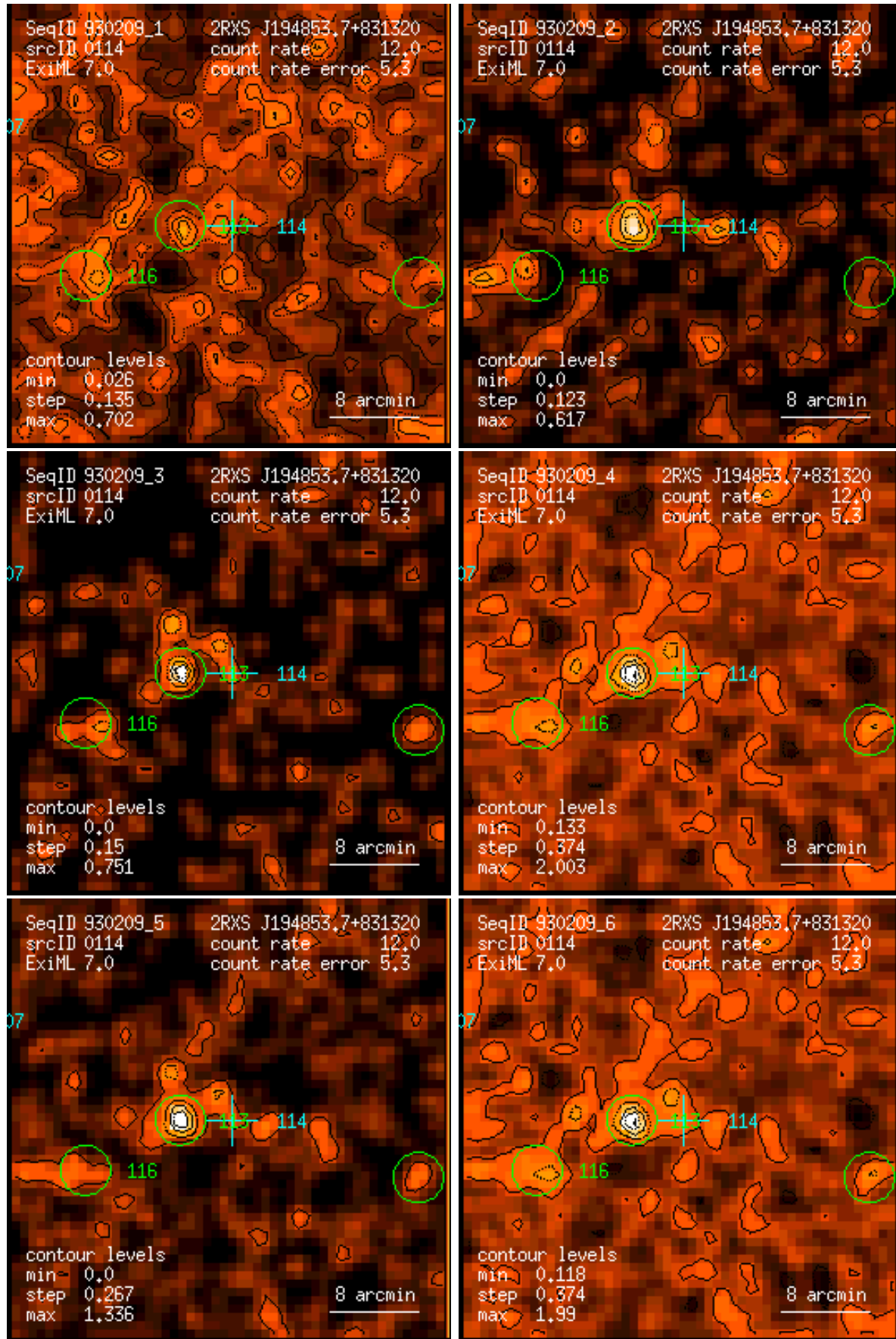
Figure 114: RASS 930209: detection 0114: band rate images, Gaussian filter: (1) PSPC channels 11 – 41, (2) 52 – 90, (3) 91 – 201, (4) 11 – 235, (5) 52 – 201, (6) 11 – 201. Broad band rates in counts/ks. Band rate contour levels in counts/ks/arcmin 2 .
