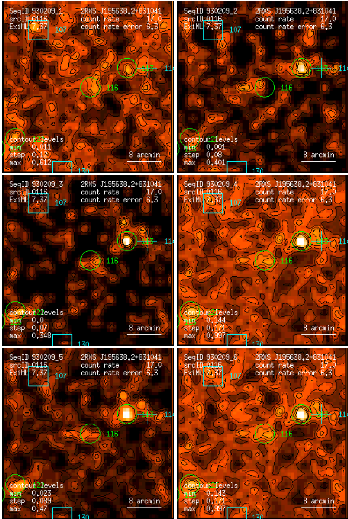
Figure 116: RASS 930209: detection 0116: band rate images, Gaussian filter: (1) PSPC channels 11 – 41, (2) 52 – 90, (3) 91 – 201, (4) 11 – 235, (5) 52 – 201, (6) 11 – 201. Broad band rates in counts/ks. Band rate contour levels in counts/ks/arcmin 2 .
