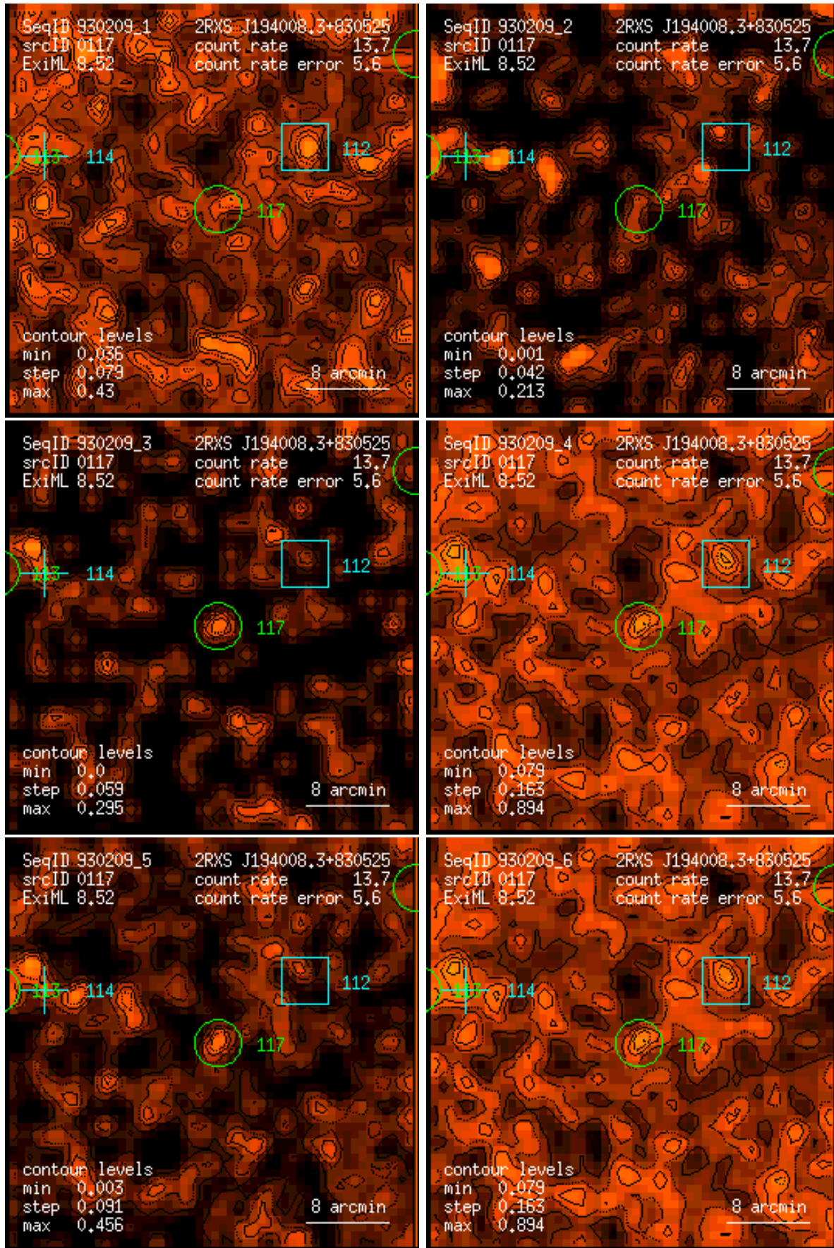
Figure 117: RASS 930209: detection 0117: band rate images, Gaussian filter: (1) PSPC channels 11 – 41, (2) 52 – 90, (3) 91 – 201, (4) 11 – 235, (5) 52 – 201, (6) 11 – 201. Broad band rates in counts/ks. Band rate contour levels in counts/ks/arcmin 2 .
