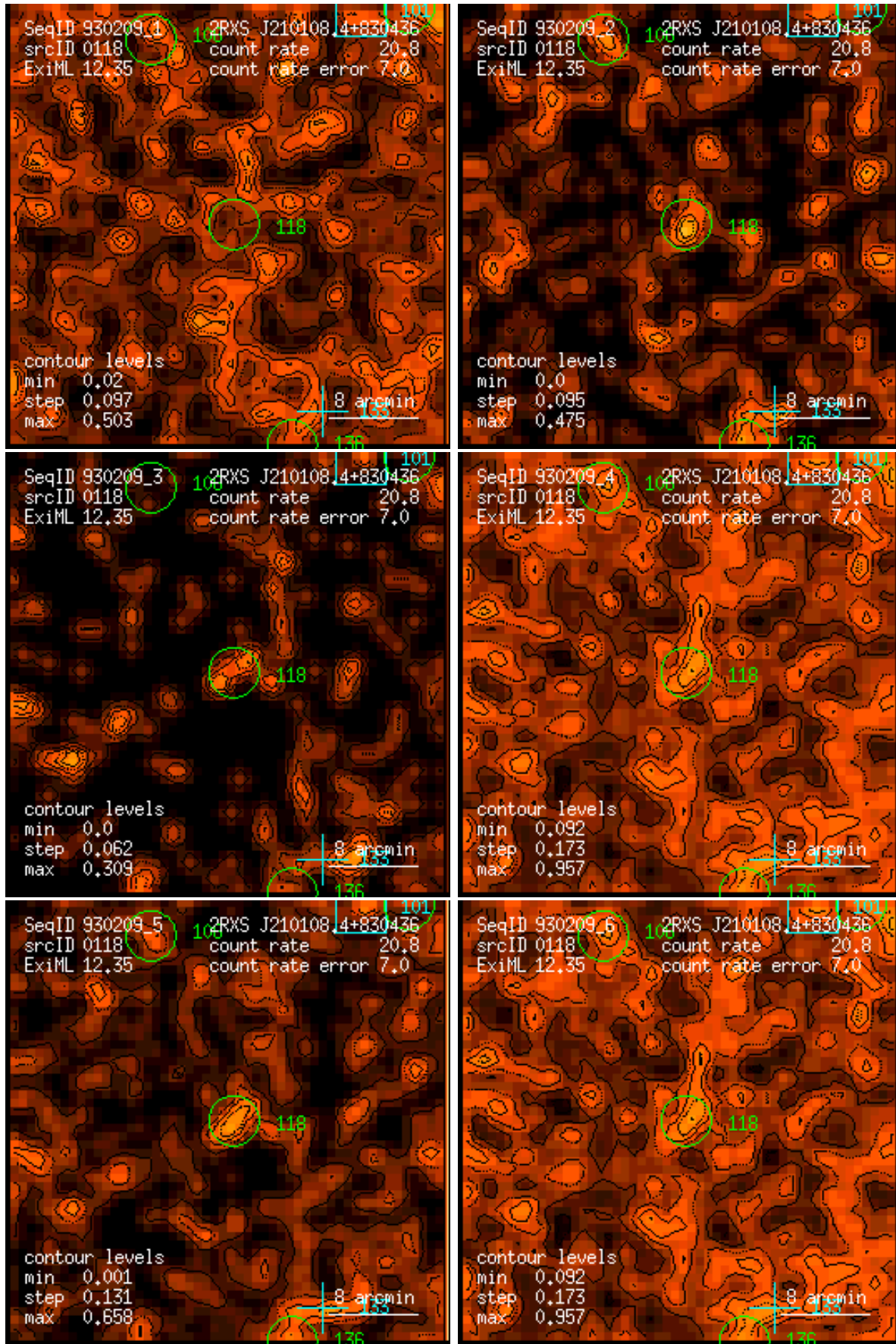
Figure 118: RASS 930209: detection 0118: band rate images, Gaussian filter: (1) PSPC channels 11 – 41, (2) 52 – 90, (3) 91 – 201, (4) 11 – 235, (5) 52 – 201, (6) 11 – 201. Broad band rates in counts/ks. Band rate contour levels in counts/ks/arcmin 2 .
