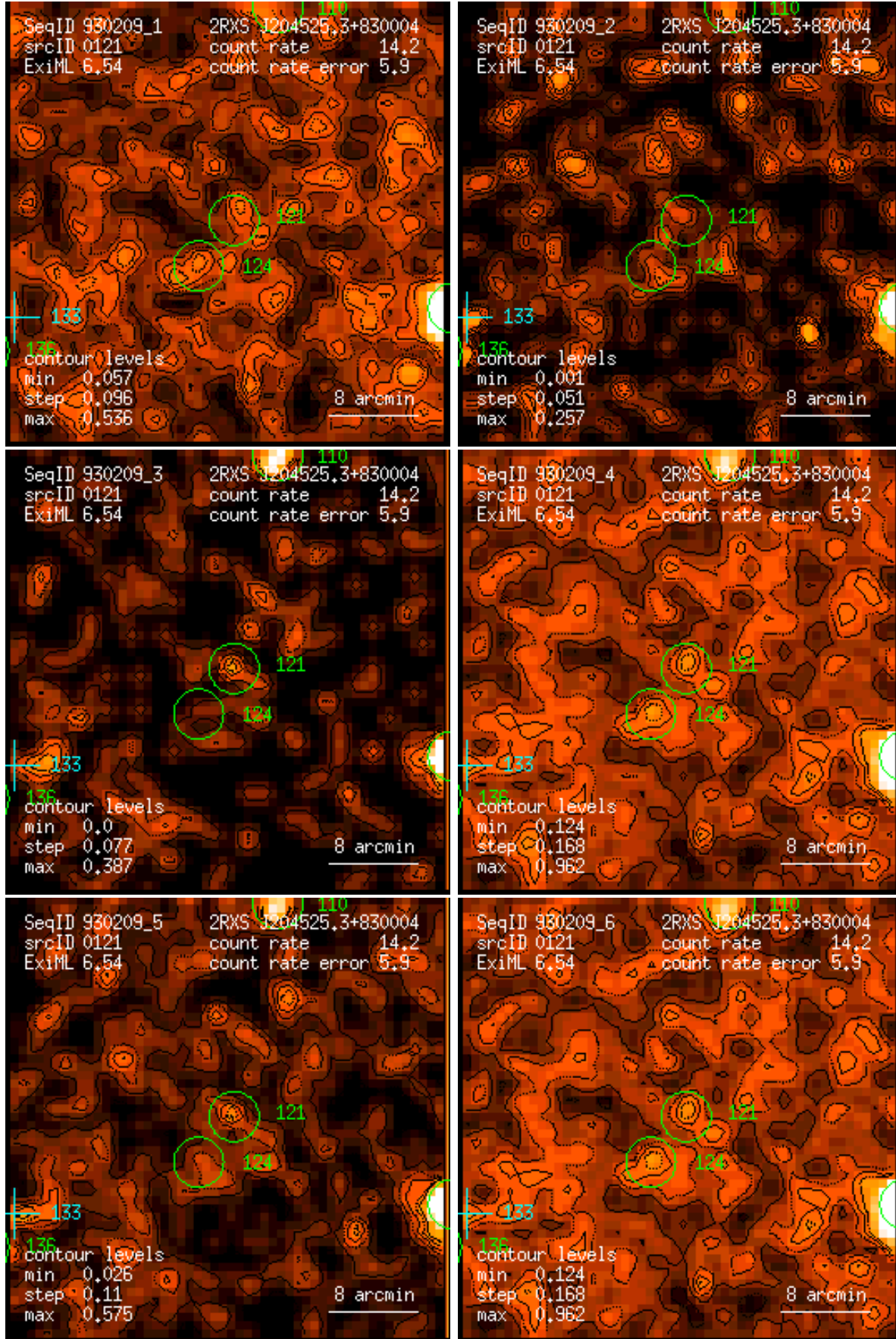
Figure 121: RASS 930209: detection 0121: band rate images, Gaussian filter: (1) PSPC channels 11 – 41, (2) 52 – 90, (3) 91 – 201, (4) 11 – 235, (5) 52 – 201, (6) 11 – 201. Broad band rates in counts/ks. Band rate contour levels in counts/ks/arcmin 2 .
