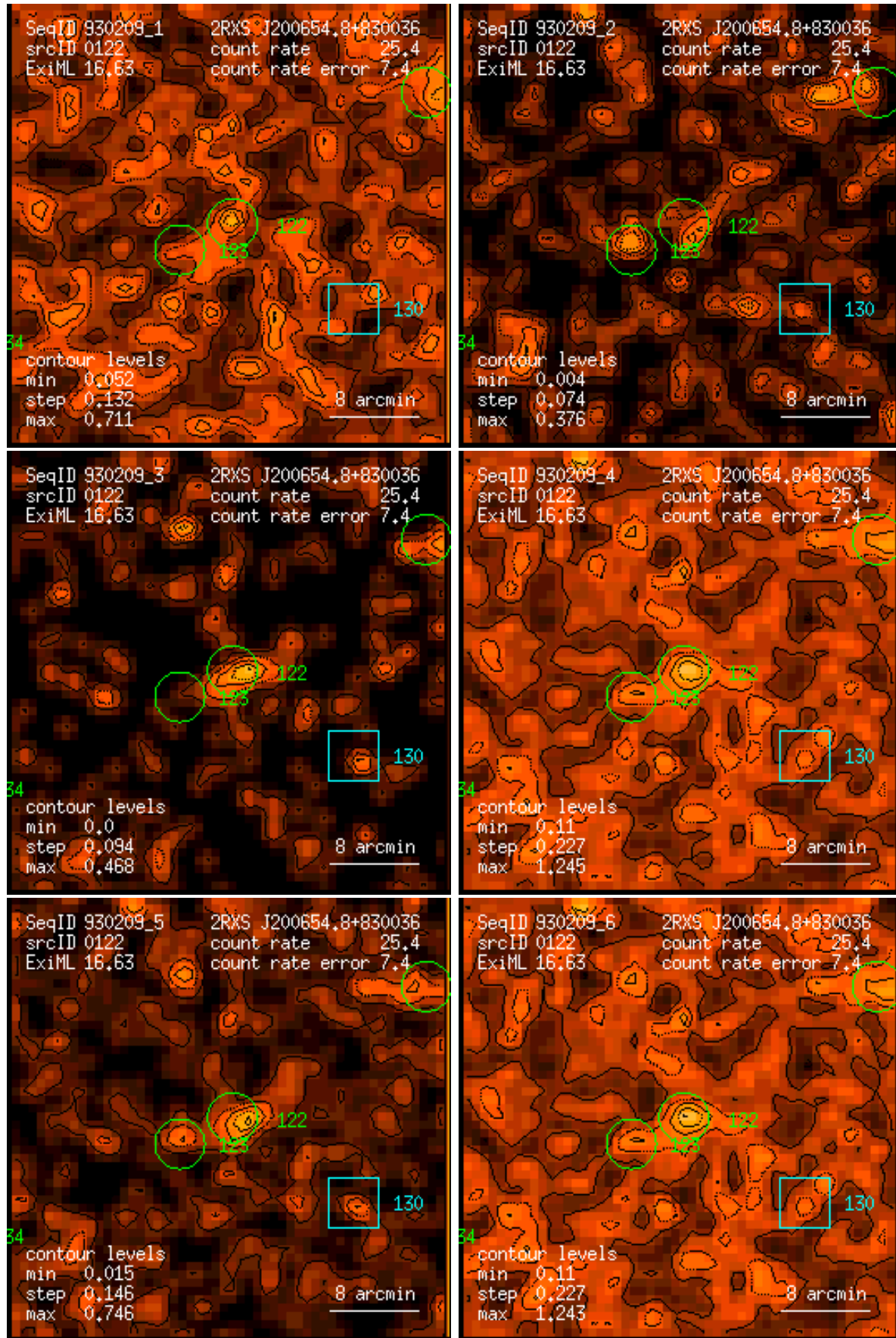
Figure 122: RASS 930209: detection 0122: band rate images, Gaussian filter: (1) PSPC channels 11 – 41, (2) 52 – 90, (3) 91 – 201, (4) 11 – 235, (5) 52 – 201, (6) 11 – 201. Broad band rates in counts/ks. Band rate contour levels in counts/ks/arcmin 2 .
