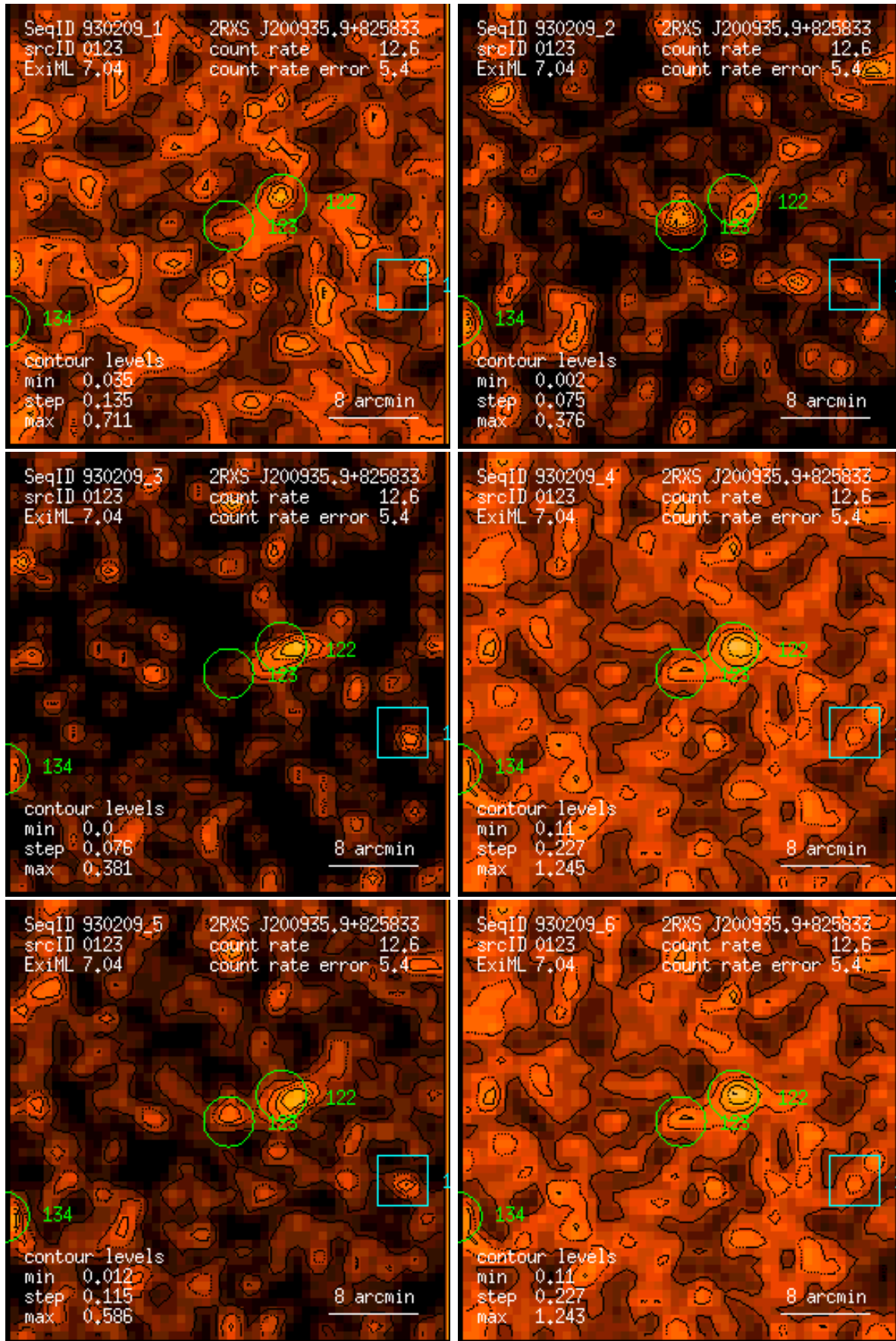
Figure 123: RASS 930209: detection 0123: band rate images, Gaussian filter: (1) PSPC channels 11 – 41, (2) 52 – 90, (3) 91 – 201, (4) 11 – 235, (5) 52 – 201, (6) 11 – 201. Broad band rates in counts/ks. Band rate contour levels in counts/ks/arcmin 2 .
