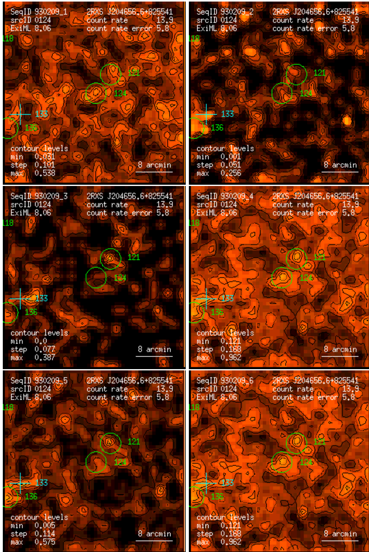
Figure 124: RASS 930209: detection 0124: band rate images, Gaussian filter: (1) PSPC channels 11 – 41, (2) 52 – 90, (3) 91 – 201, (4) 11 – 235, (5) 52 – 201, (6) 11 – 201. Broad band rates in counts/ks. Band rate contour levels in counts/ks/arcmin 2 .
