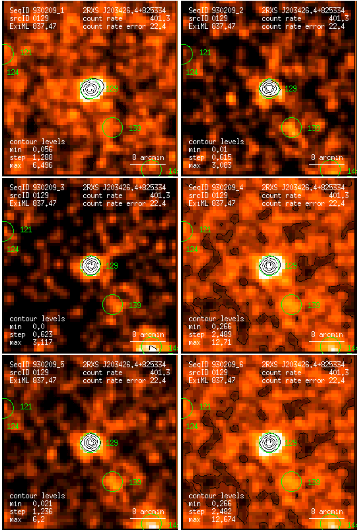
Figure 129: RASS 930209: detection 0129: band rate images, Gaussian filter: (1) PSPC channels 11 – 41, (2) 52 – 90, (3) 91 – 201, (4) 11 – 235, (5) 52 – 201, (6) 11 – 201. Broad band rates in counts/ks. Band rate contour levels in counts/ks/arcmin 2 .
