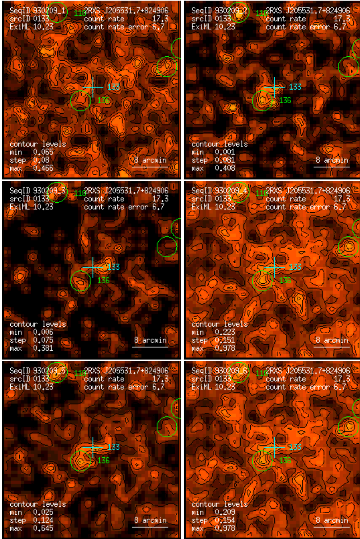
Figure 133: RASS 930209: detection 0133: band rate images, Gaussian filter: (1) PSPC channels 11 – 41, (2) 52 – 90, (3) 91 – 201, (4) 11 – 235, (5) 52 – 201, (6) 11 – 201. Broad band rates in counts/ks. Band rate contour levels in counts/ks/arcmin 2 .
