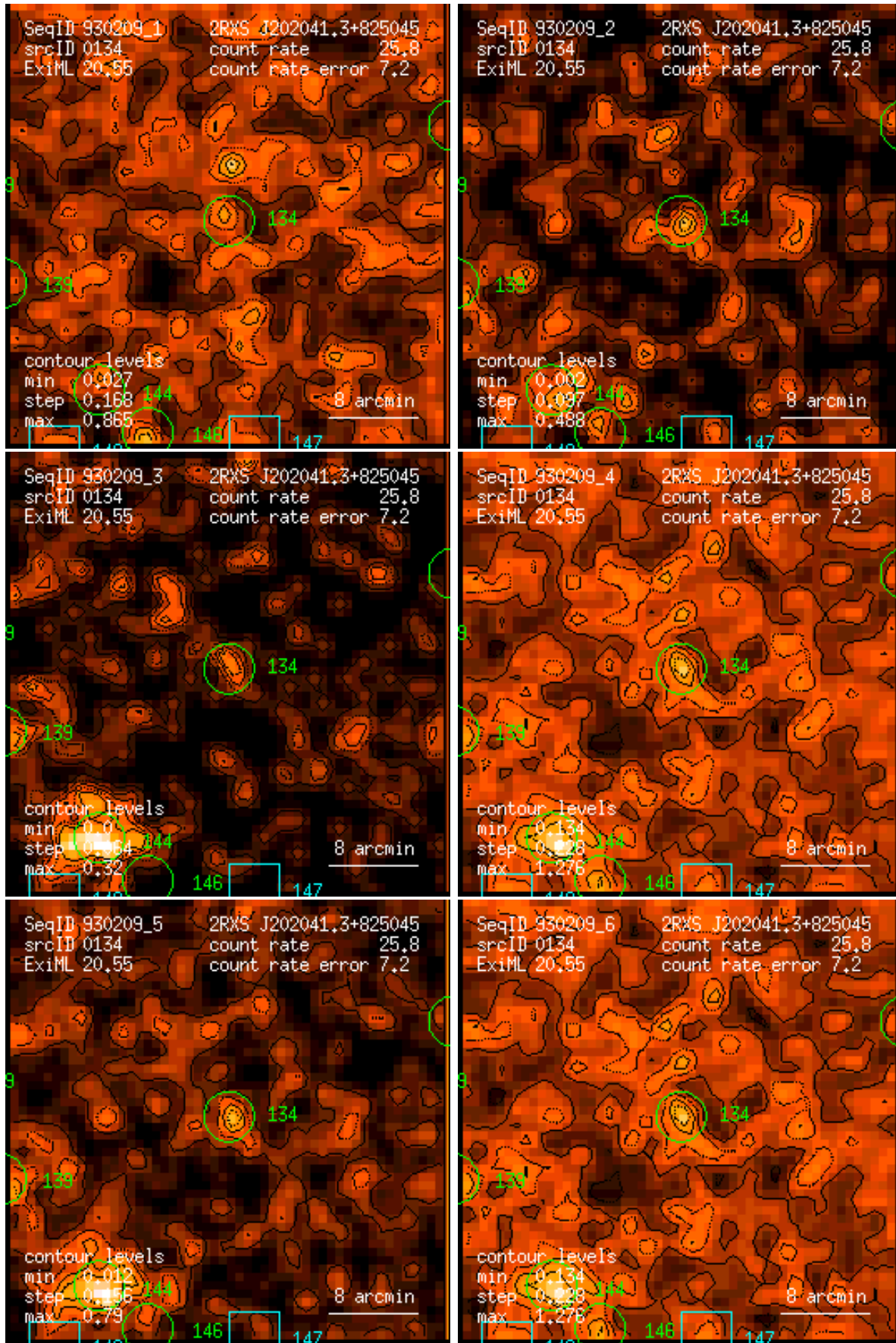
Figure 134: RASS 930209: detection 0134: band rate images, Gaussian filter: (1) PSPC channels 11 – 41, (2) 52 – 90, (3) 91 – 201, (4) 11 – 235, (5) 52 – 201, (6) 11 – 201. Broad band rates in counts/ks. Band rate contour levels in counts/ks/arcmin 2 .
