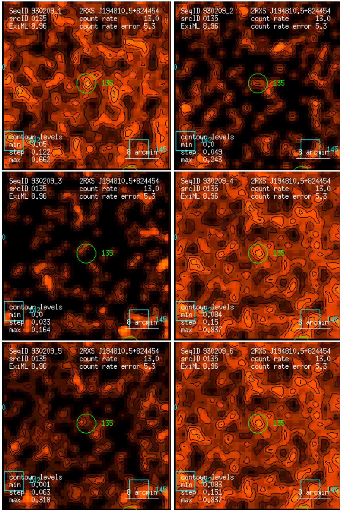
Figure 135: RASS 930209: detection 0135: band rate images, Gaussian filter: (1) PSPC channels 11 – 41, (2) 52 – 90, (3) 91 – 201, (4) 11 – 235, (5) 52 – 201, (6) 11 – 201. Broad band rates in counts/ks. Band rate contour levels in counts/ks/arcmin 2 .
