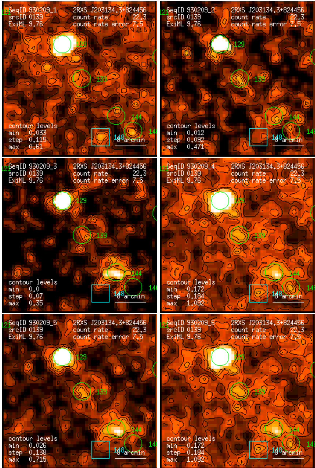
Figure 139: RASS 930209: detection 0139: band rate images, Gaussian filter: (1) PSPC channels 11 – 41, (2) 52 – 90, (3) 91 – 201, (4) 11 – 235, (5) 52 – 201, (6) 11 – 201. Broad band rates in counts/ks. Band rate contour levels in counts/ks/arcmin 2 .
