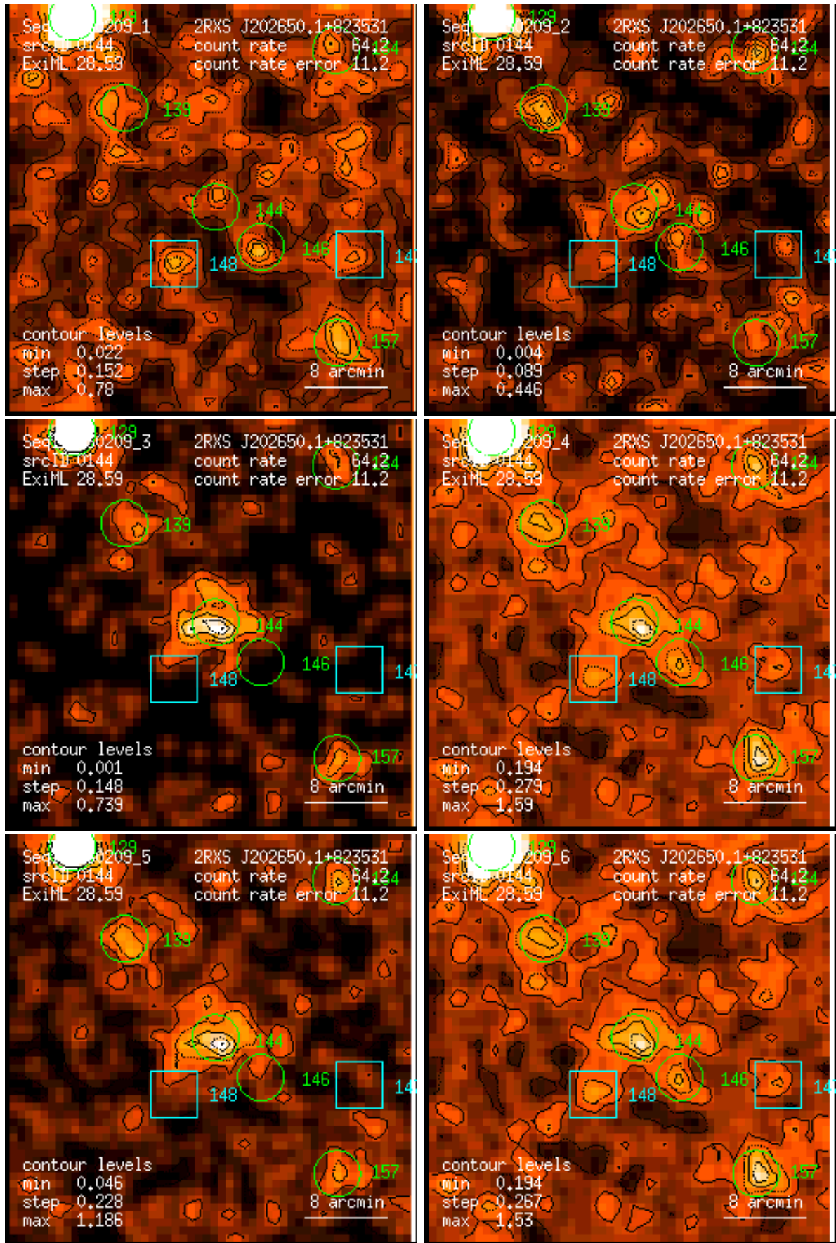
Figure 144: RASS 930209: detection 0144: band rate images, Gaussian filter: (1) PSPC channels 11 – 41, (2) 52 – 90, (3) 91 – 201, (4) 11 – 235, (5) 52 – 201, (6) 11 – 201. Broad band rates in counts/ks. Band rate contour levels in counts/ks/arcmin 2 .
