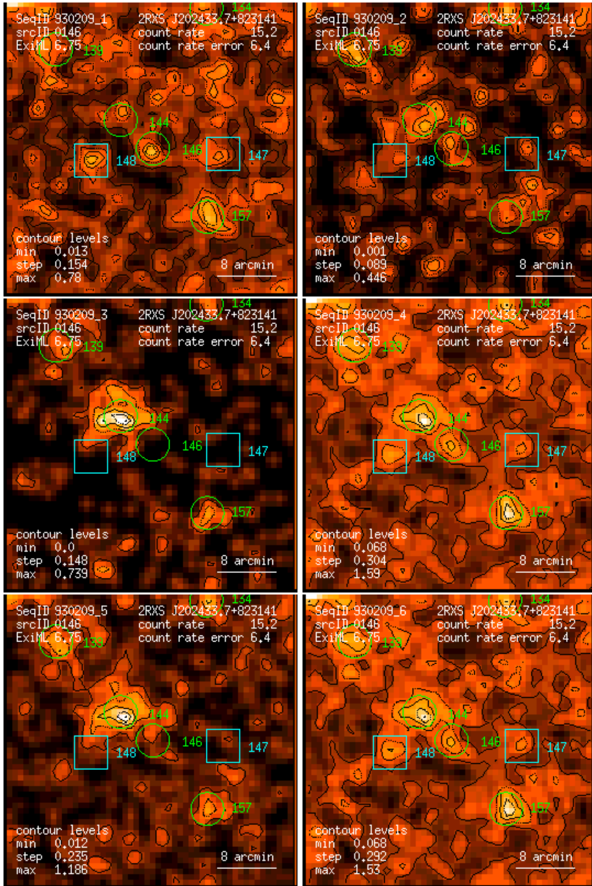
Figure 146: RASS 930209: detection 0146: band rate images, Gaussian filter: (1) PSPC channels 11 – 41, (2) 52 – 90, (3) 91 – 201, (4) 11 – 235, (5) 52 – 201, (6) 11 – 201. Broad band rates in counts/ks. Band rate contour levels in counts/ks/arcmin 2 .
