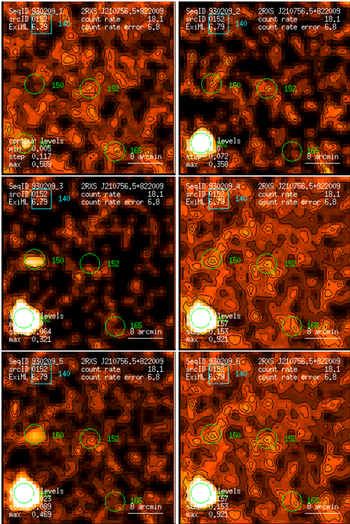
Figure 152: RASS 930209: detection 0152: band rate images, Gaussian filter: (1) PSPC channels 11 – 41, (2) 52 – 90, (3) 91 – 201, (4) 11 – 235, (5) 52 – 201, (6) 11 – 201. Broad band rates in counts/ks. Band rate contour levels in counts/ks/arcmin 2 .
