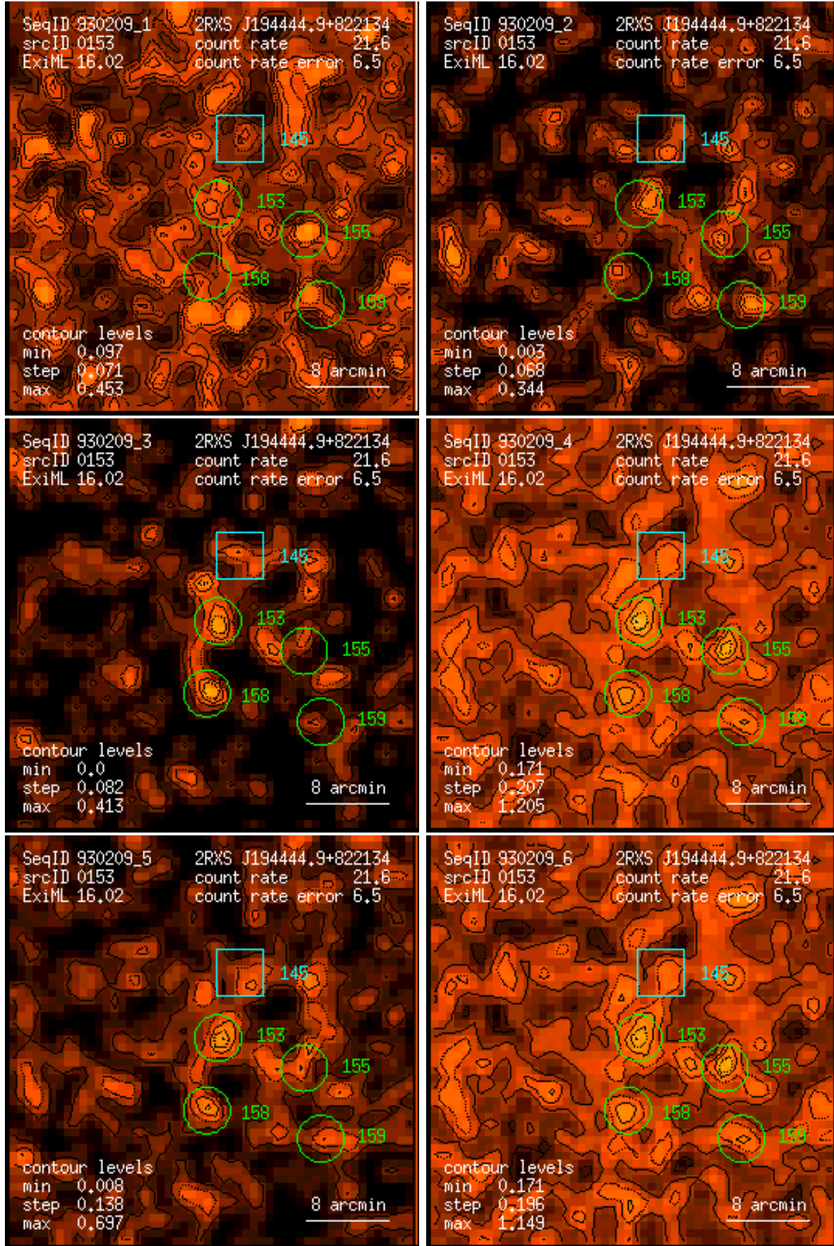
Figure 153: RASS 930209: detection 0153: band rate images, Gaussian filter: (1) PSPC channels 11 – 41, (2) 52 – 90, (3) 91 – 201, (4) 11 – 235, (5) 52 – 201, (6) 11 – 201. Broad band rates in counts/ks. Band rate contour levels in counts/ks/arcmin 2 .
