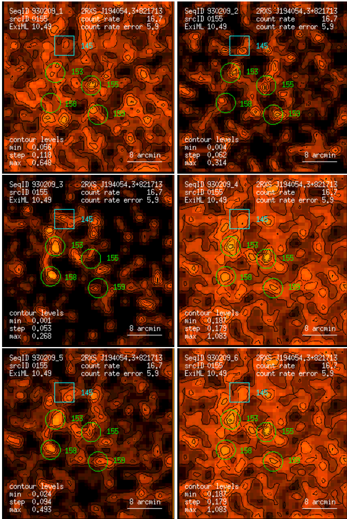
Figure 155: RASS 930209: detection 0155: band rate images, Gaussian filter: (1) PSPC channels 11 – 41, (2) 52 – 90, (3) 91 – 201, (4) 11 – 235, (5) 52 – 201, (6) 11 – 201. Broad band rates in counts/ks. Band rate contour levels in counts/ks/arcmin 2 .
