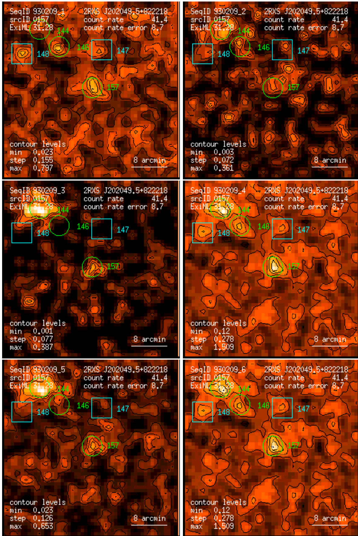
Figure 157: RASS 930209: detection 0157: band rate images, Gaussian filter: (1) PSPC channels 11 – 41, (2) 52 – 90, (3) 91 – 201, (4) 11 – 235, (5) 52 – 201, (6) 11 – 201. Broad band rates in counts/ks. Band rate contour levels in counts/ks/arcmin 2 .
