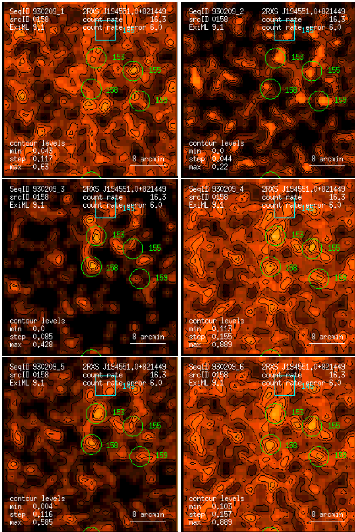
Figure 158: RASS 930209: detection 0158: band rate images, Gaussian filter: (1) PSPC channels 11 – 41, (2) 52 – 90, (3) 91 – 201, (4) 11 – 235, (5) 52 – 201, (6) 11 – 201. Broad band rates in counts/ks. Band rate contour levels in counts/ks/arcmin 2 .
